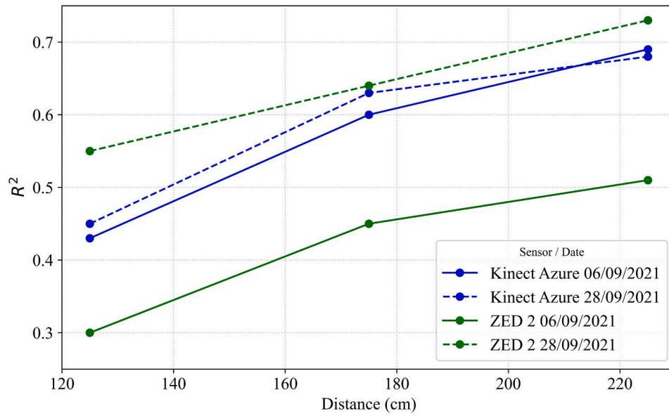
Fig. 8. Scanning performance by distance, comparison between ZED 2 and Kinect Azure camera.
