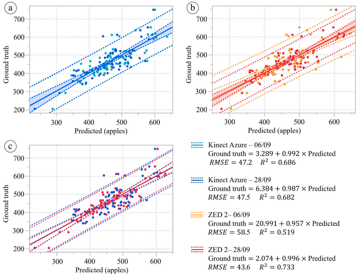
Fig. 9. Comparison of the dispersion graph and regression lines in three different situations, all them at 225 cm from the sensor with respect to the axis of the row of trees: a) Azure Kinect at two different dates; b) ZED 2 at two different dates; c) one week before the harvest, ZED 2 and Azure Kinect. Confidence and prediction bands are represented by dotted lines.
