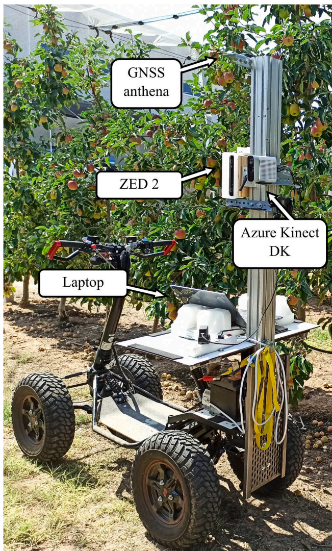
Fig. 2. Orchard scanning equipment.
