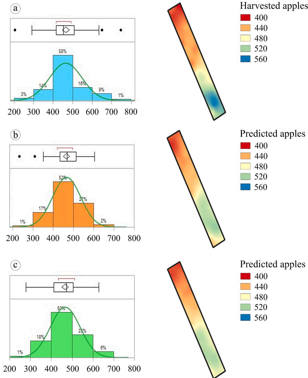
Fig. 10. Comparison of the distribution of predicted and actual values with their corresponding orchard block-level yield maps: a) ground truth; b) predictions with the Azure Kinect sensor; c) predictions with the ZED 2 sensor.
