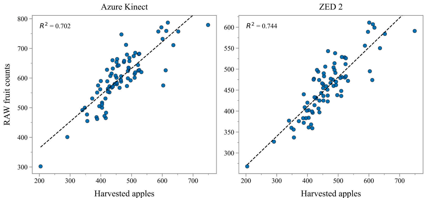
Fig. 7. Relationship between harvested apples (ground truth) and the raw fruit counts obtained using the load estimation pipeline; Azure Kinect (left) and ZED 2 (right).
