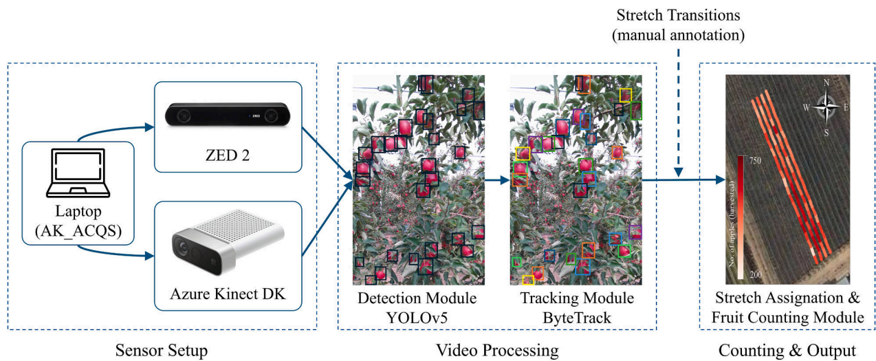
Fig. 4. Flow chart from video capture to orchard block-level yield map.
