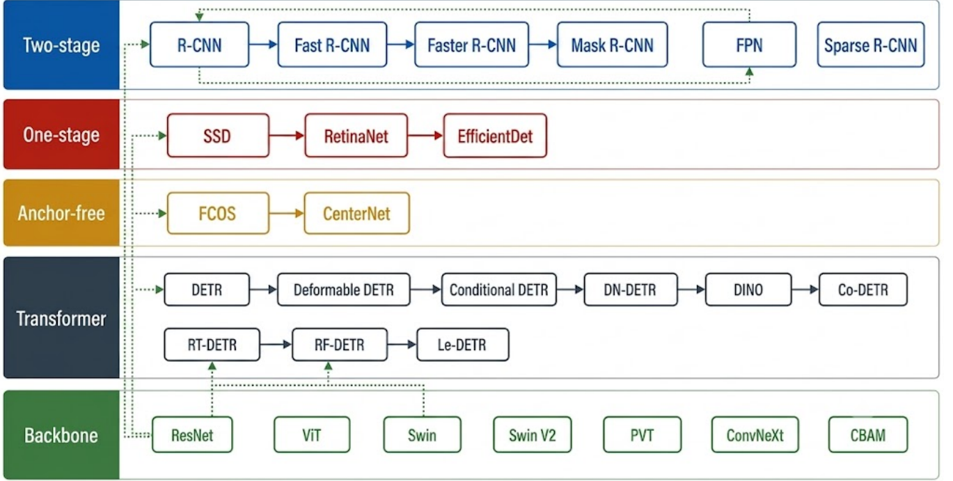
Fig. 5. Genealogy of the RGB detector paradigms and the inheritance of ideas between them: the two-stage line (R-CNN through Sparse R-CNN), the one-stage line (SSD, RetinaNet, EfficientDet), the anchor-free line (FCOS, CenterNet), and the transformer line (DETR through the real-time DETR variants).
