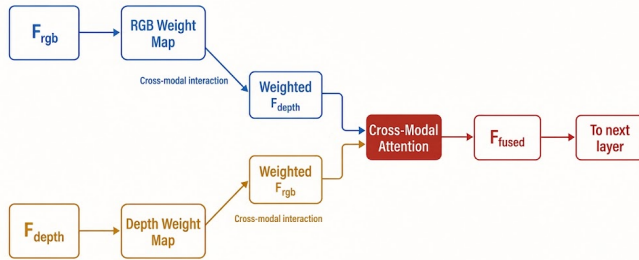
Fig. 8. The cross-modal attention mechanism that recurs across the strongest RGB-D methods (for example SA-Gate, CIR-Net, CMX): each modality generates a weighting map that gates the other before fusion, so a faulty depth measurement can be suppressed rather than allowed to contaminate the joint representation.
