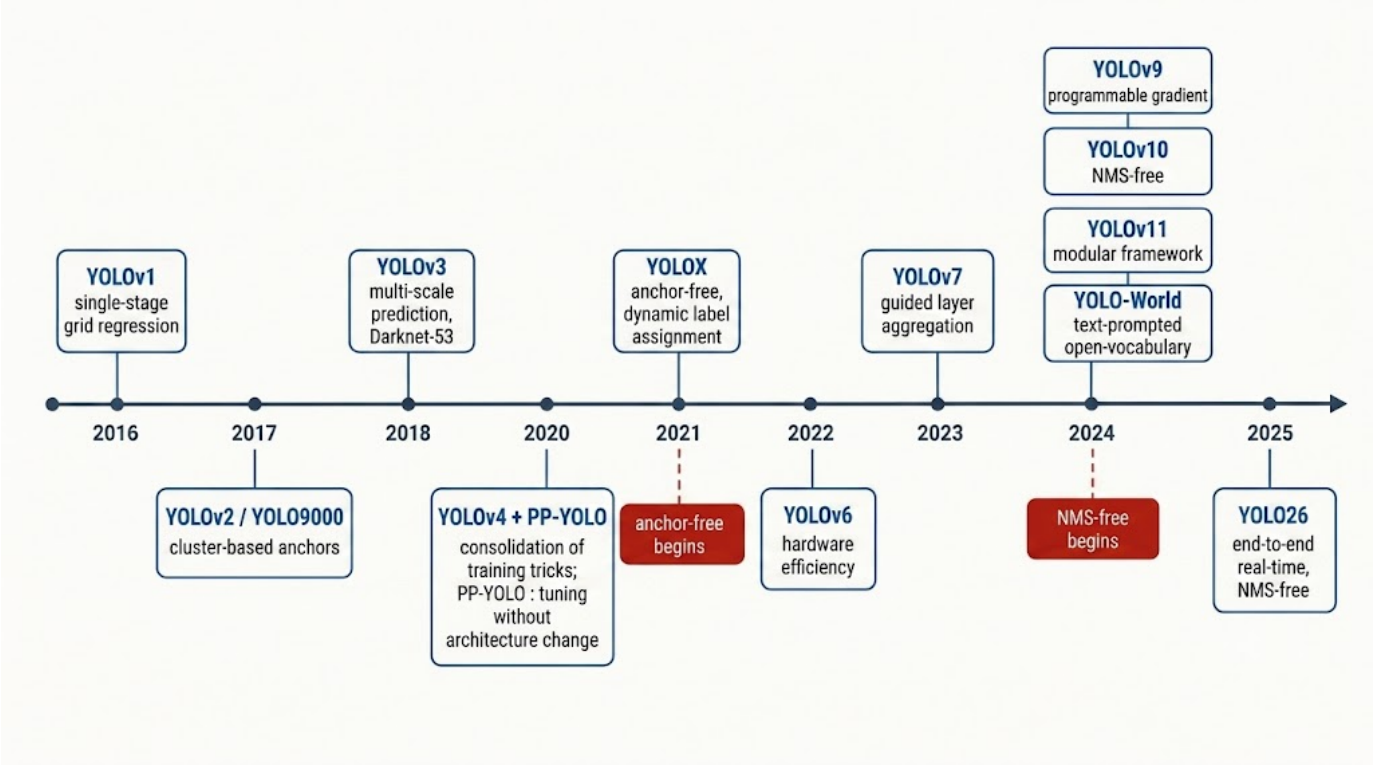
Fig. 6. Timeline of the YOLO family and its principal architectural markers, from the single-pass grid regression of YOLOv1 (2016) through anchor-free decoupled heads, re-parameterization, and the NMS-free end-to-end designs of YOLOv10 and YOLO26.
