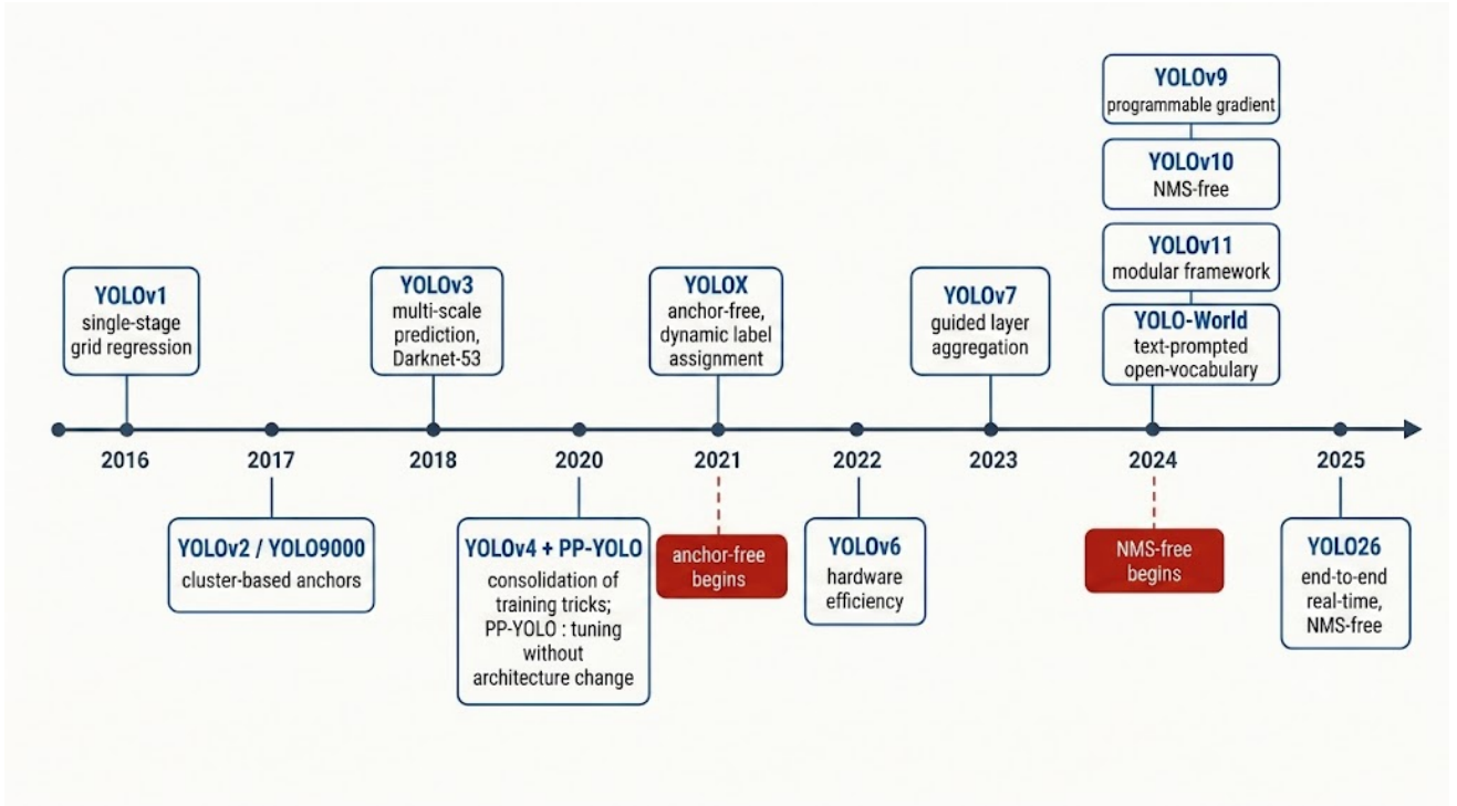
Figure 5: Timeline of the YOLO family and its principal architectural markers, from the single-pass grid regression of YOLOv1 (2016) through anchor-free decoupled heads, re-parameterization, and the NMS-free end-to-end designs of YOLOv10 and YOLO26.
