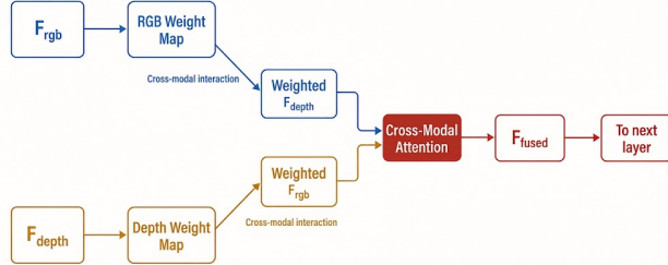
Figure 7: The cross-modal attention mechanism that recurs across the strongest RGB-D methods (e.g. SA-Gate, CIR-Net, CMX): each modality generates a weighting map that gates the other before fusion, so a faulty depth measurement can be suppressed rather than allowed to contaminate the joint representation.
