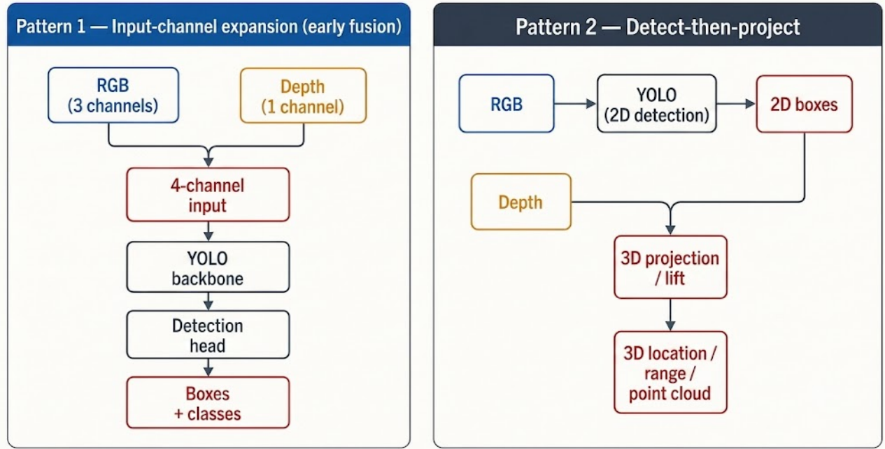
Figure 8: The two recurring patterns for integrating YOLO with depth. Pattern one expands the input to four channels and fuses at the input (Expandable YOLO), which Ophoff et al. find is dominated by intermediate fusion; pattern two detects in 2D and then projects or refines in 3D on a reduced region (FusionVision, YOLOv8-URE).
