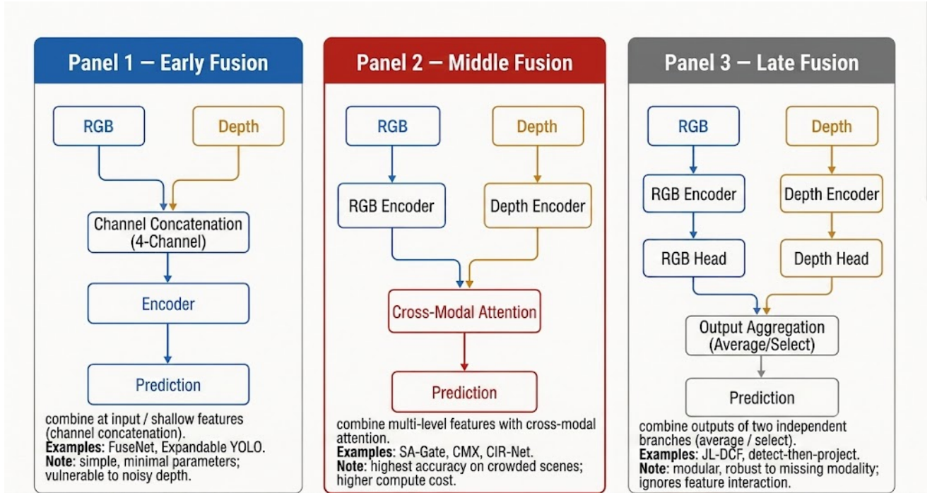
Figure 6: The three fusion locations that structure the RGB-D literature. Early fusion concatenates colour and depth at the input (e.g. FuseNet, Expandable YOLO); middle/feature fusion learns modality-specific representations before exchanging them at selected scales; late fusion combines predictions and supports an explicit RGB fallback.
