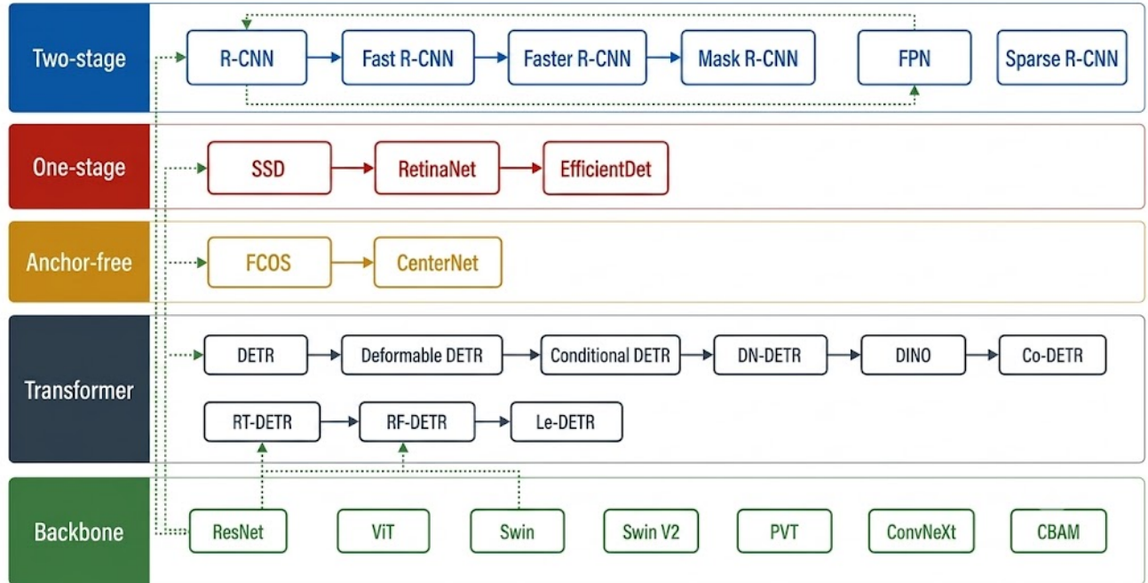
Figure 4: Genealogy of the RGB detector paradigms and the inheritance of ideas between them: the two-stage line (R-CNN through Sparse R-CNN), the one-stage line (SSD, RetinaNet, EfficientDet), the anchor-free line (FCOS, CenterNet), and the transformer line (DETR through the real-time DETR variants).
