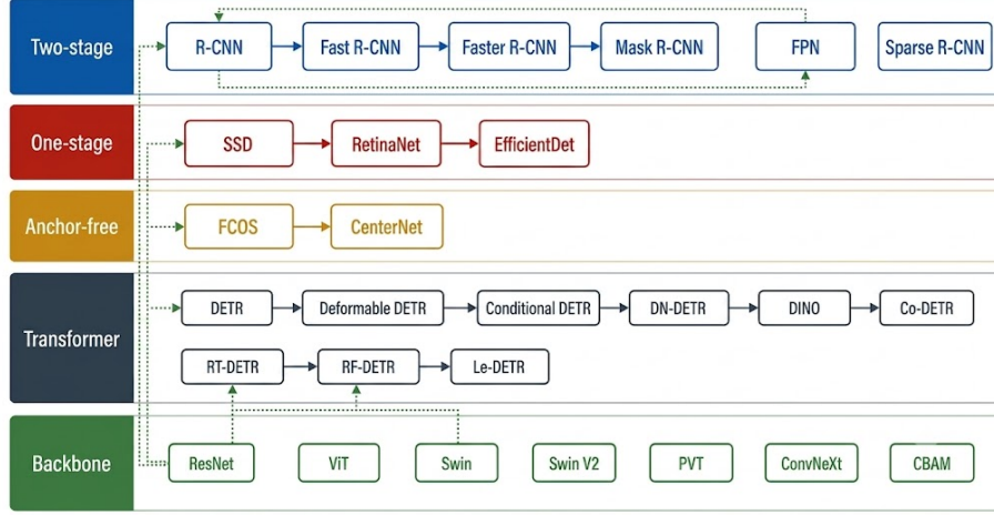
Figure 4: Genealogy of the RGB detector paradigms and the inheritance of ideas between them: the two-stage line (R-CNN through Sparse R-CNN), the one-stage line (SSD, RetinaNet, EfficientDet), the anchor-free line (FCOS, CenterNet), and the transformer line (DETR through the real-time DETR variants).
