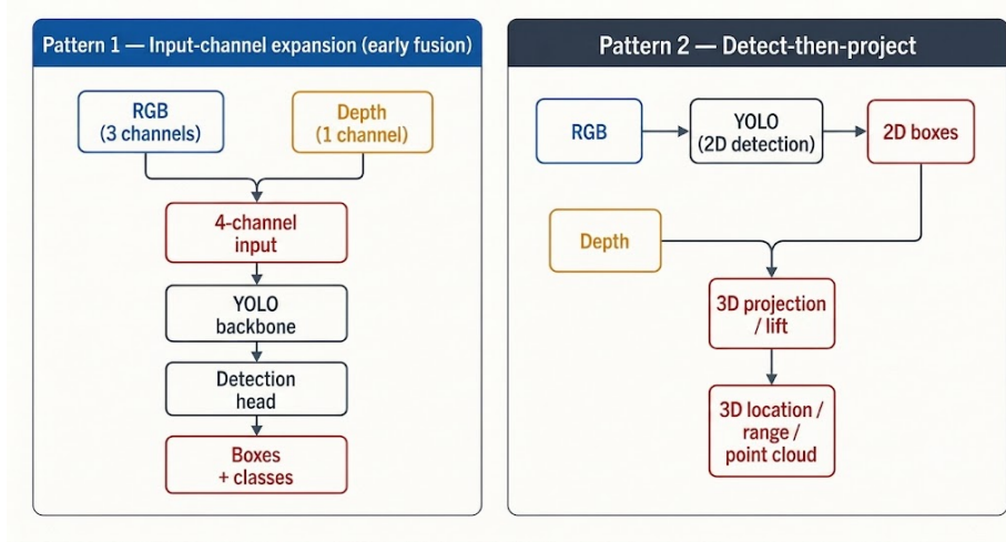
Figure 8: The two recurring patterns for integrating YOLO with depth. Pattern one expands the input to four channels and fuses at the input (Expandable YOLO), which Ophoff et al. find is dominated by intermediate fusion; pattern two detects in 2D and then projects or refines in 3D on a reduced region (FusionVision, YOLOv8-URE).
