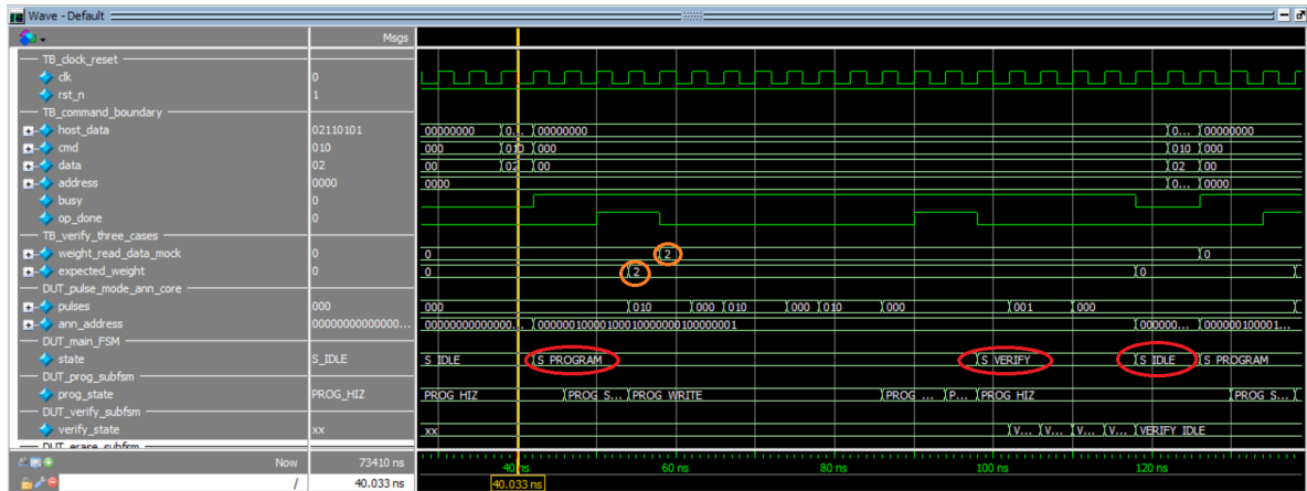
Figure 6.1: Closed-loop recovery (Match case): The readback data equals the expected weight (2). The FSM naturally exits the S\_PROGRAM \rightarrow S\_VERIFY loop and returns to S\_IDLE .
