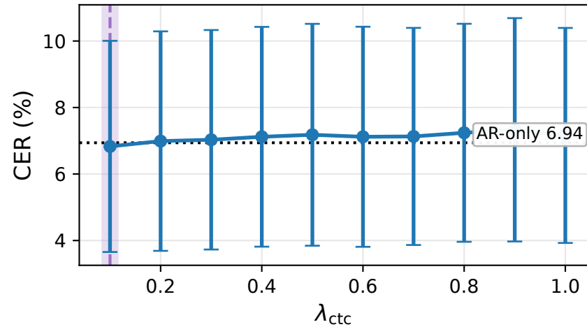
Downstream AR CER vs \lambda_{\text{ctc}}
