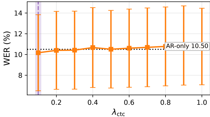
Downstream AR WER vs \lambda_{\text{ctc}}
