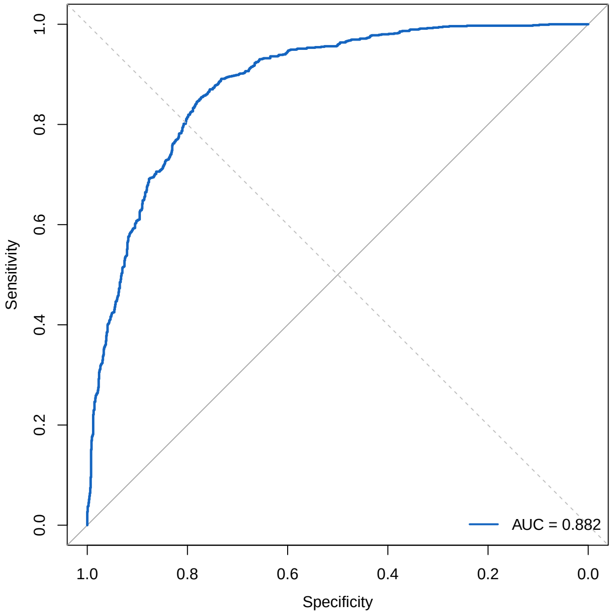
Gambar 7. ROC Curve – Regresi Logistik
