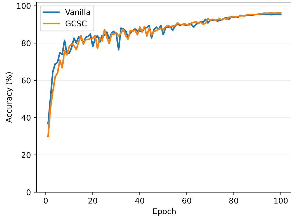
Validation accuracy
