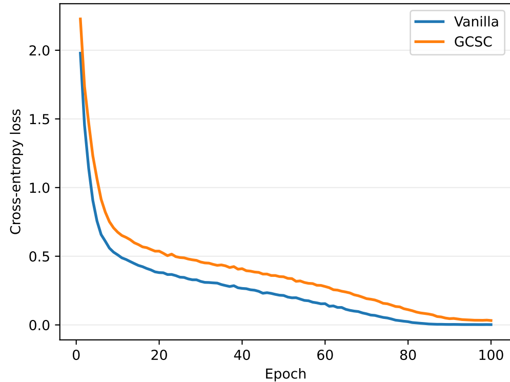
Training loss
