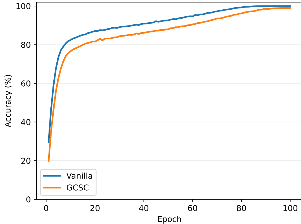
Training accuracy
