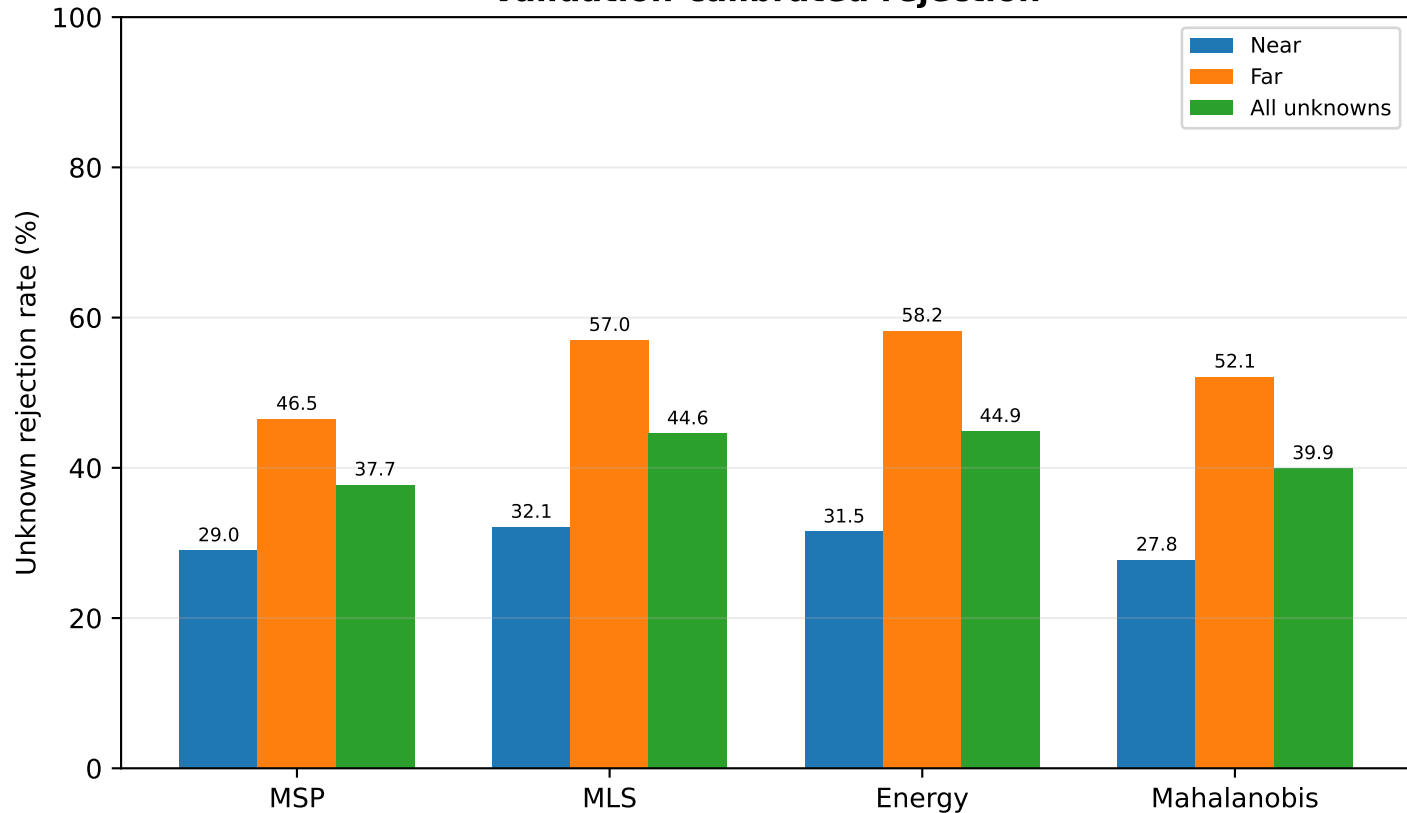
Validation-calibrated rejection
