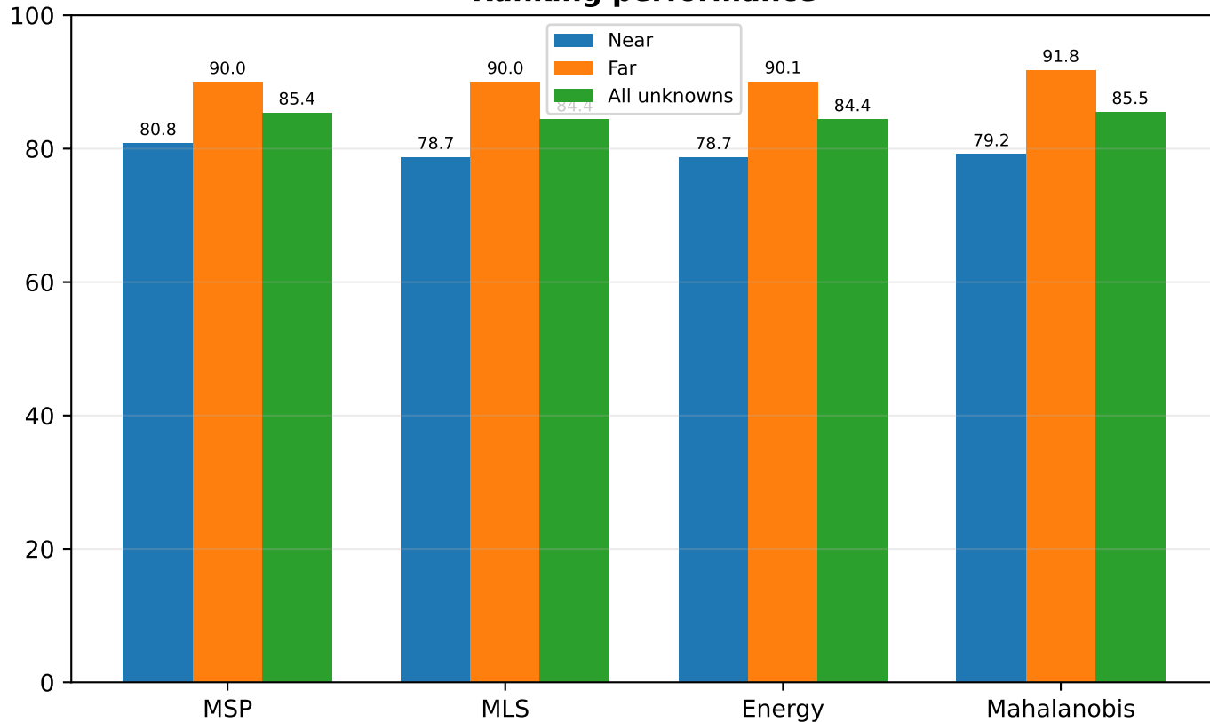
Ranking performance
