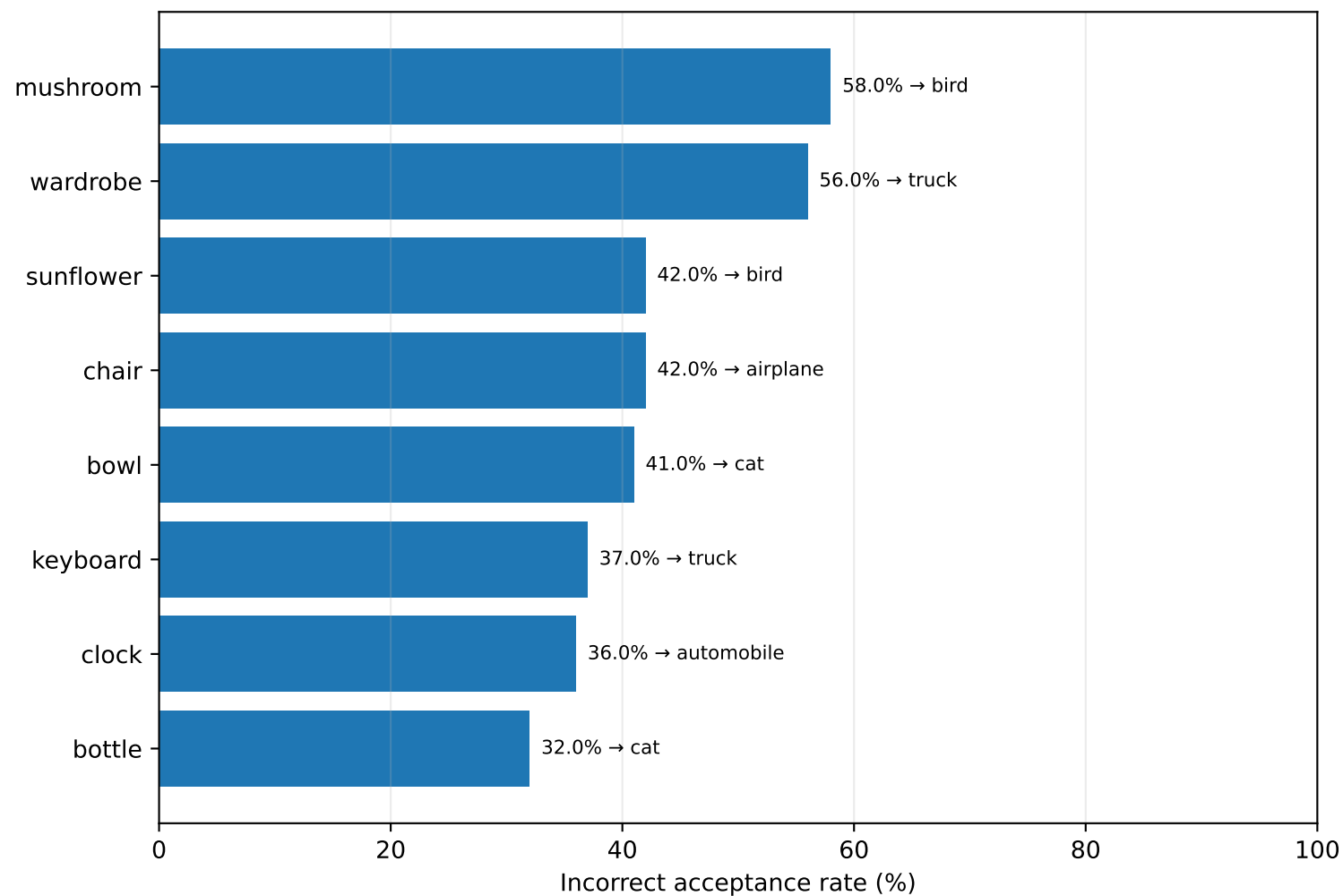
Far unknowns
