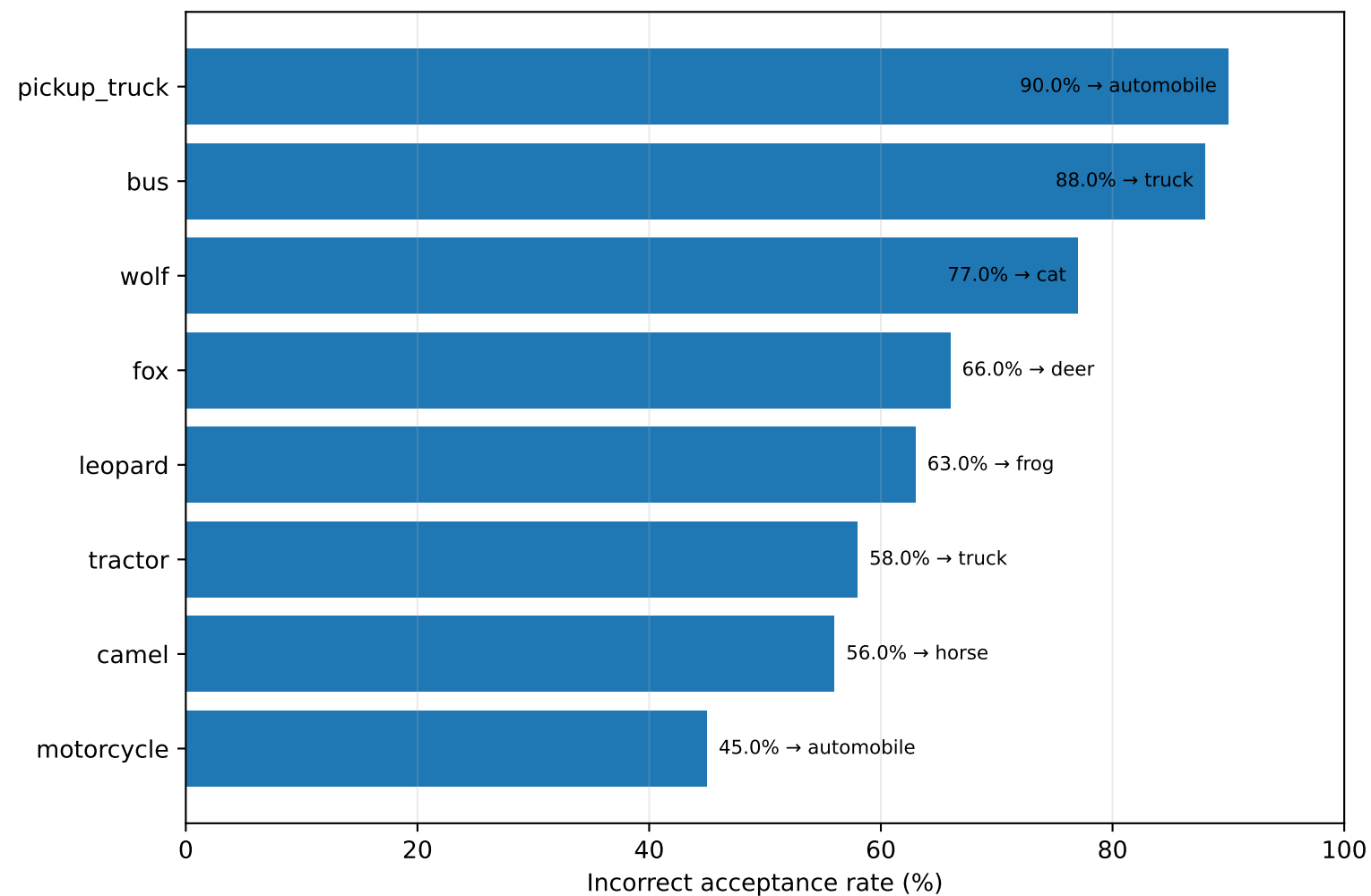
Near unknowns
