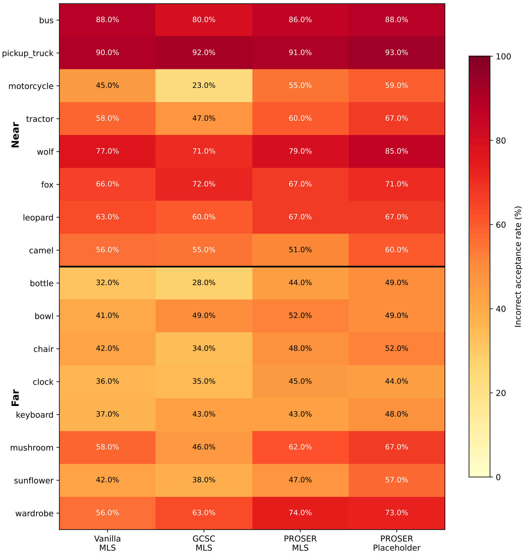
Classwise Unknown Acceptance Across Models and Scores
