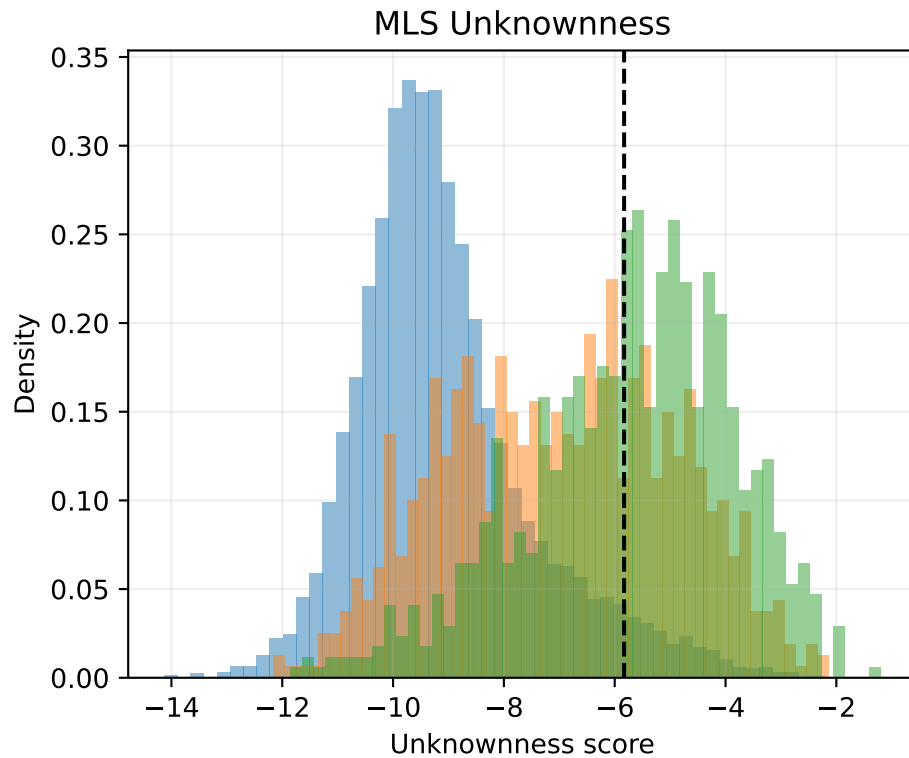
Vanilla Model: Known and Unknown Score Distributions
