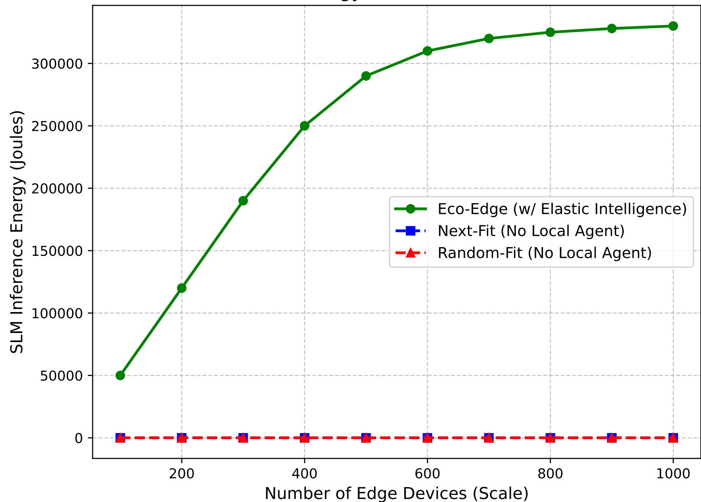
SLM Inference Energy Overhead vs. Network Scale
