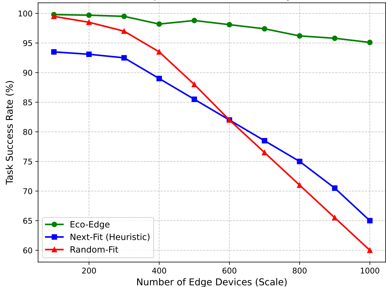
Task Completion Rate under Heavy Load
