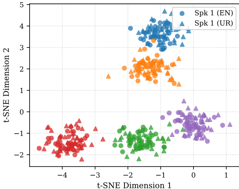
(a) Baseline Linear Fusion (FOP_MAV) Cross-Lingual Identity Clustering ( \bar{S} = 0.482 )
