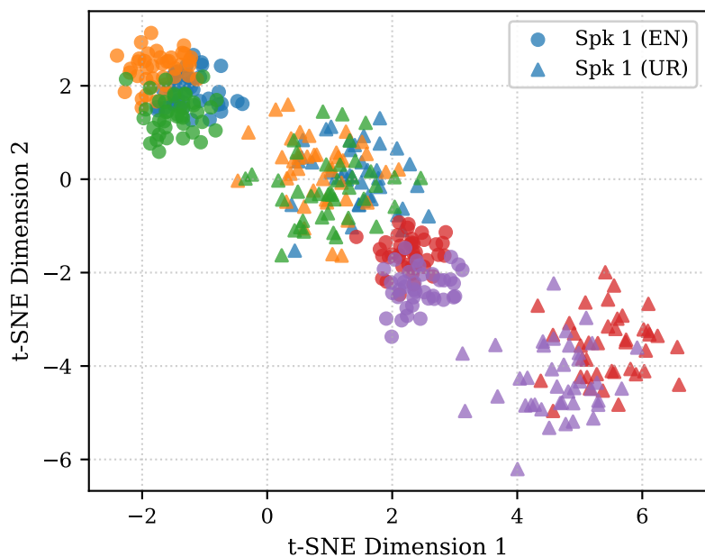
(b) MultiBranch Cross-Attention Cross-Lingual Domain Shift ( S = 0.214 )
