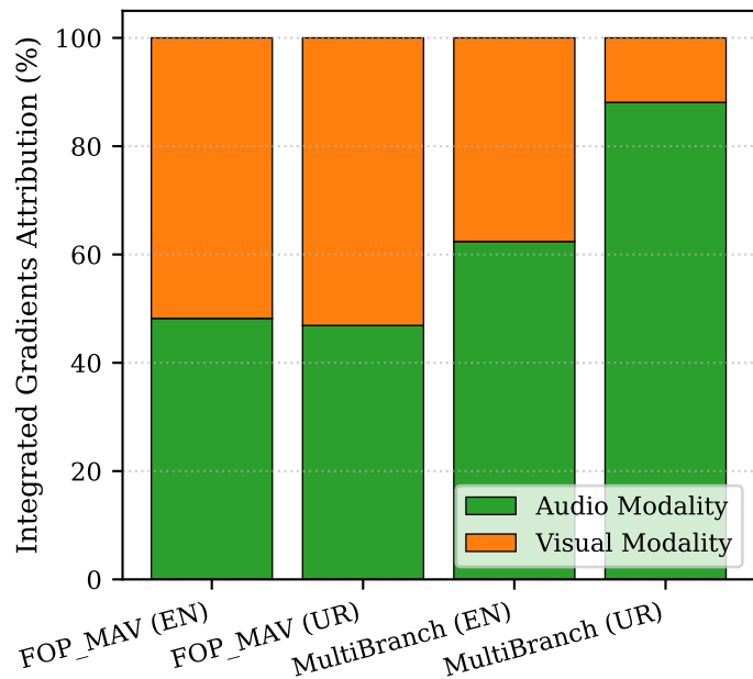
(b) Modality Attribution & Visual Anchor Status
