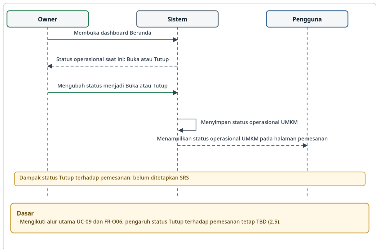
Gambar 12. Sequence Diagram Owner Mengatur Status Operasional UMKM (UC-09, FR-006)
