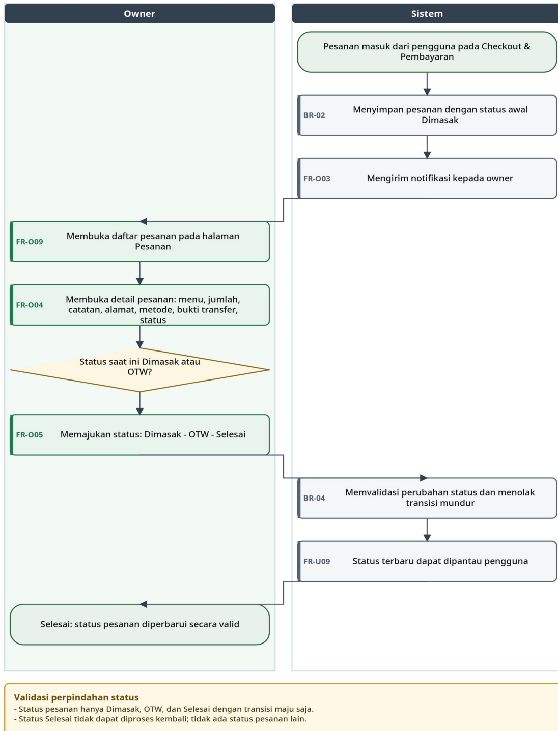
Gambar 4. Workflow Owner UC-08 - Memproses Pesanan Masuk
