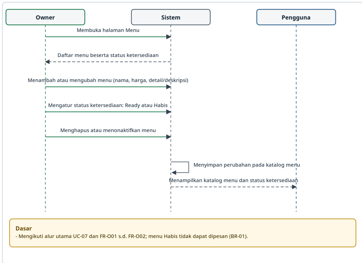
Gambar 11. Sequence Diagram Owner Mengelola Katalog Menu (UC-07, FR-001 dan FR-002)
