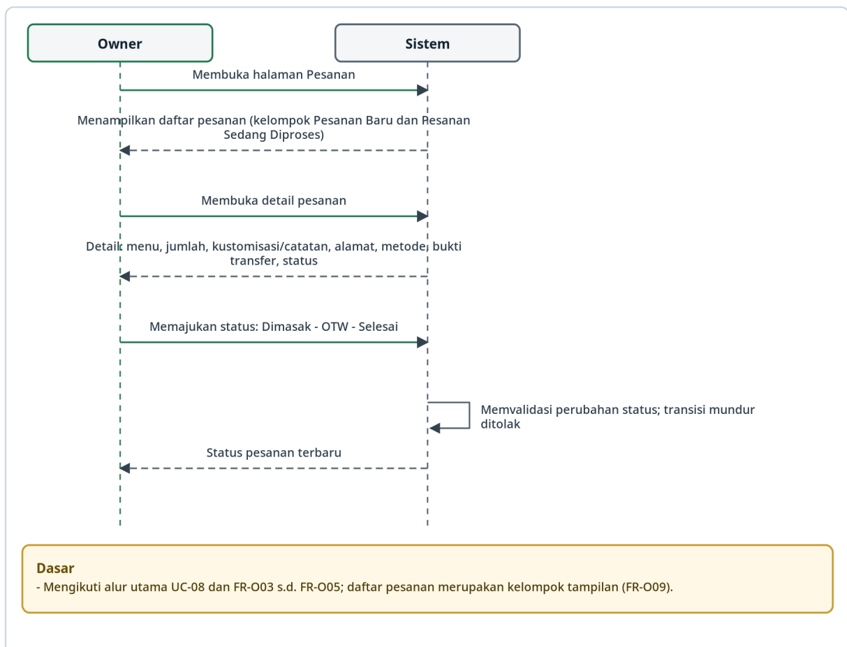
Gambar 10. Sequence Diagram Owner Memproses Pesanan Masuk (UC-08, FR-O03 s.d. FR-O05)
