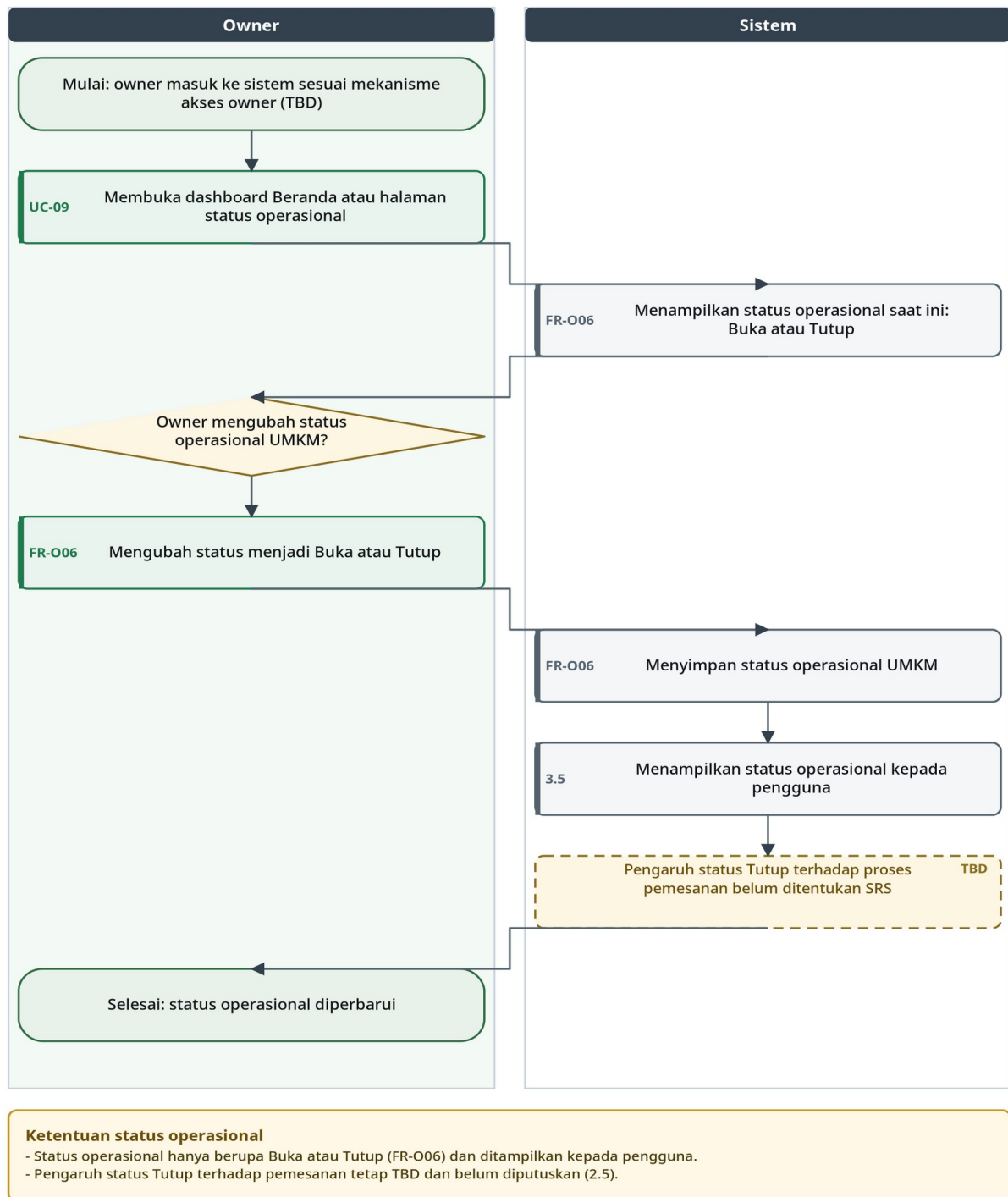
Gambar 5. Workflow Owner UC-09 - Mengatur Status Operasional UMKM
