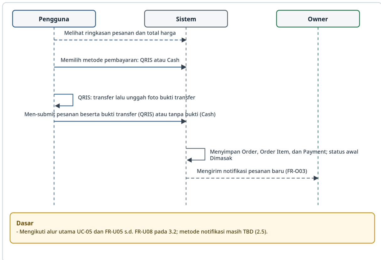
Gambar 9. Sequence Diagram Checkout & Pembayaran (UC-05, FR-U05 s.d. FR-U08)
