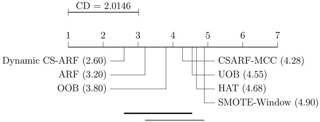
Figure 4: Critical Difference (CD) diagram for the post-hoc Nemenyi test. Classifiers connected by the same horizontal line have no significant performance difference at the Nemenyi post-hoc level ( \alpha = 0.05 ).
