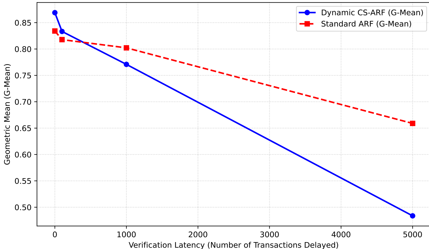
Performance Degradation under Delayed Labels (ULB Dataset)
