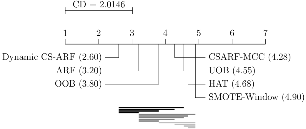
Figure 4: Critical Difference (CD) diagram for the post-hoc Nemenyi test. Classifiers connected by the same horizontal line have no significant performance difference at \alpha = 0.05 .
