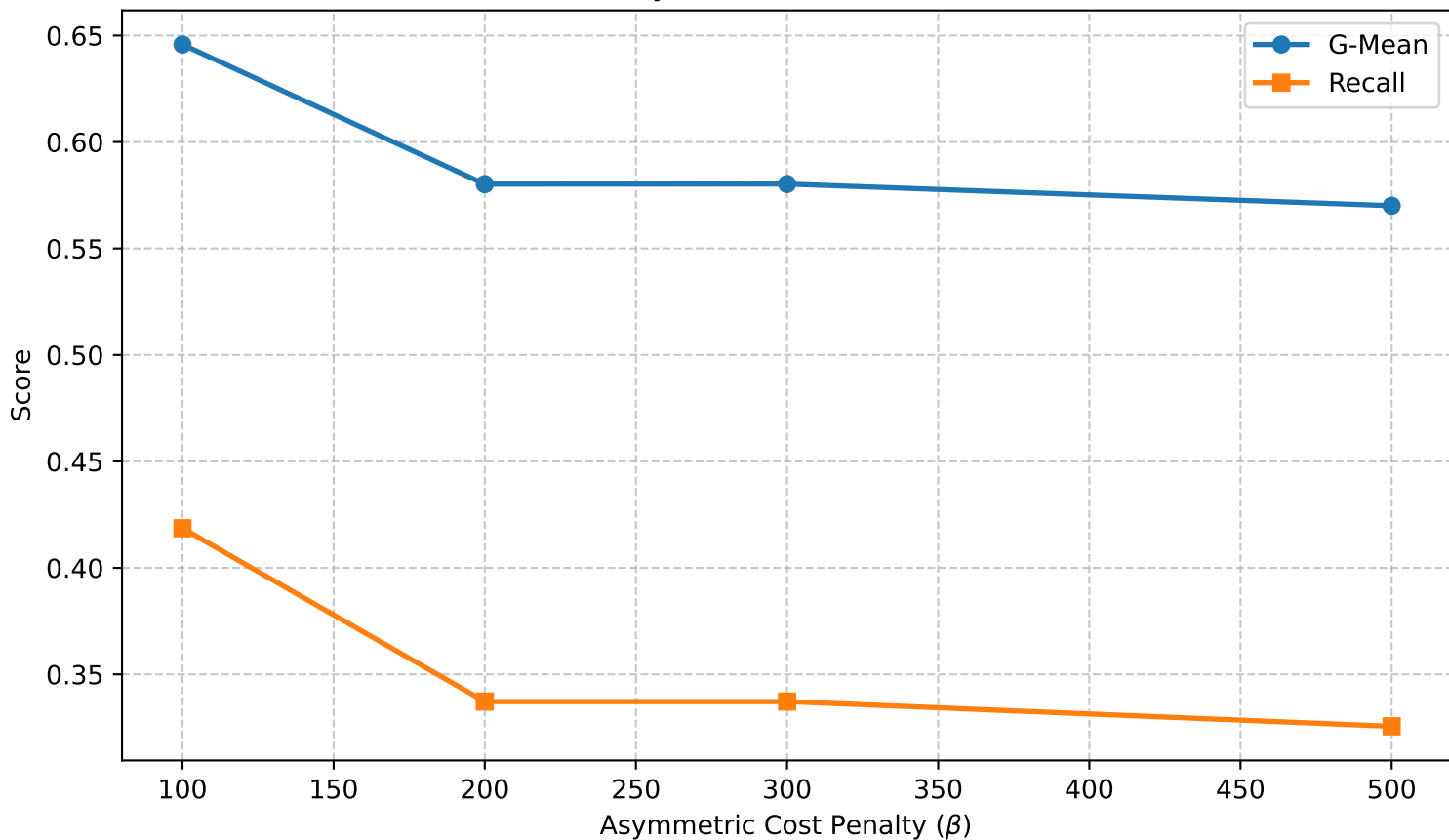
Ablation Study on ULB Dataset (50k Subset)
