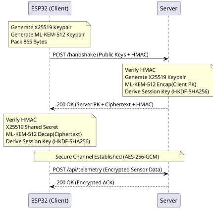
Fig. 2. Fig. 2. Authenticated hybrid X25519/ML-KEM-512 handshake over persistent TCP, showing public-parameter authentication, server encapsulation, HKDF binding, and AES-GCM telemetry activation.
