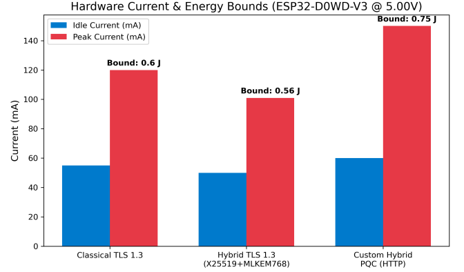
Fig. 5. Peak current profiles and absolute maximum energy bounds for a single full handshake on the ESP32-D0WD-V3 at 5.00V.
