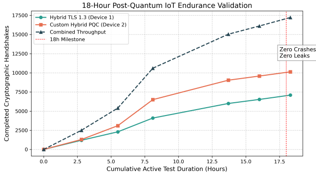
Fig. 4. Cumulative throughput and stability of the 18-hour hybrid post-quantum endurance evaluation.
