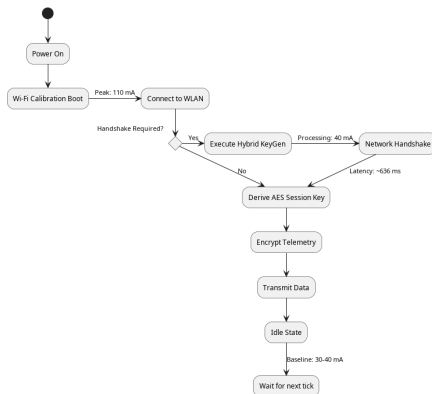
Fig. 3. Power Consumption Lifecycle of the ESP32
