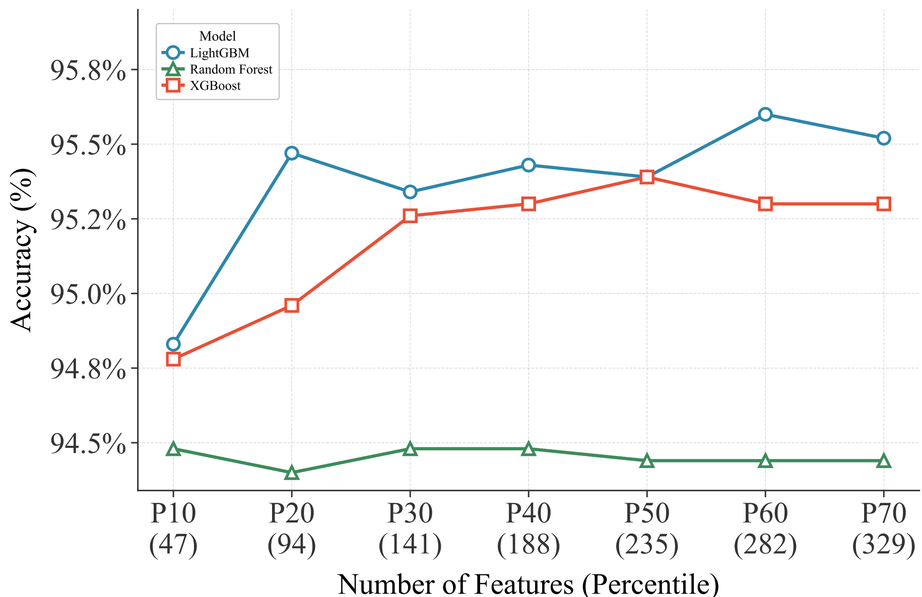
Figure 1. Accuracy of LightGBM, XGBoost, and Random Forest across feature subsets selected at increasing percentile thresholds (P10-P70), with the corresponding number of selected features shown in parentheses.
