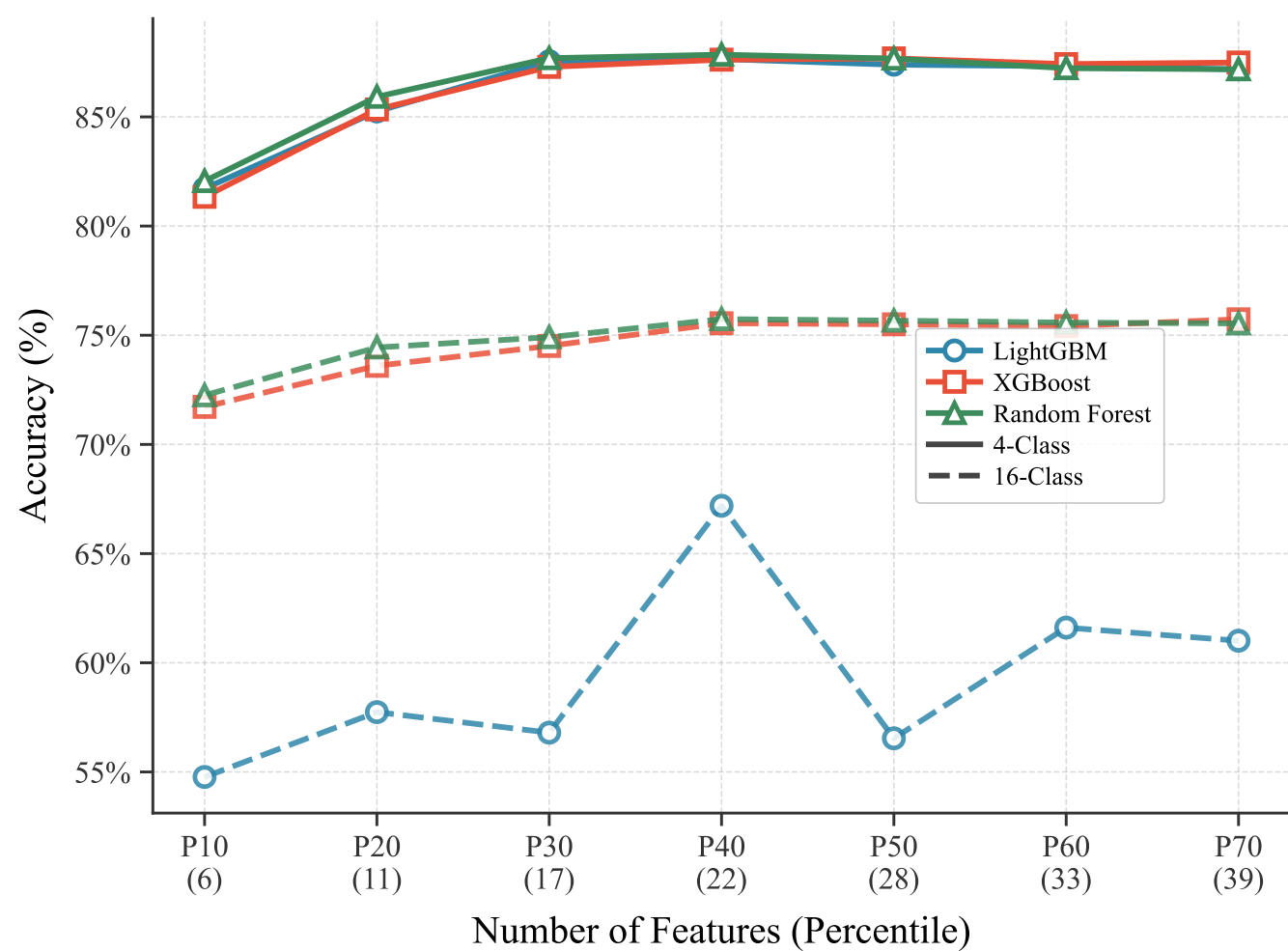
Figure 3. Accuracy (left) and macro F1-score (right) of LightGBM, XGBoost, and Random Forest under the 4-class (solid line) and 16-class (dashed line) classification scenarios, across feature subsets selected at increasing percentile thresholds (P10-P70); numbers in parentheses indicate the corresponding number of selected features.
