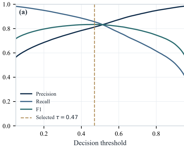
Decision metric
