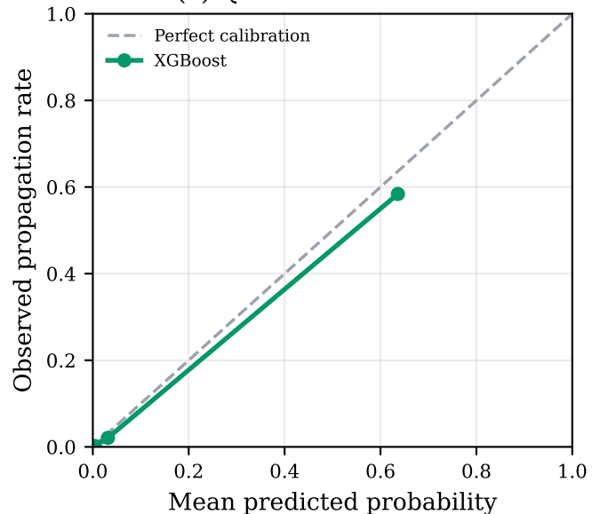
(c) Quantile Calibration
