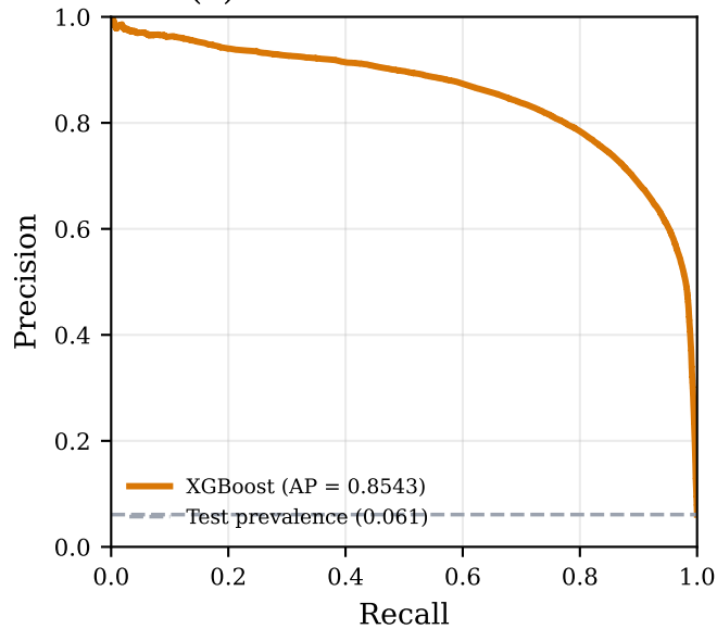
(b) Precision-Recall Curve
