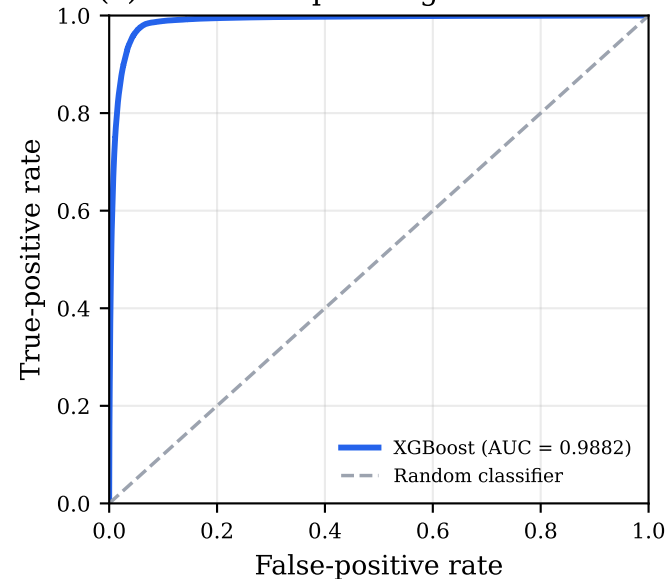
(a) Receiver Operating Characteristic
