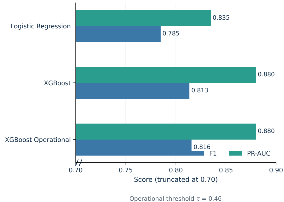
(a) Validation model comparison
