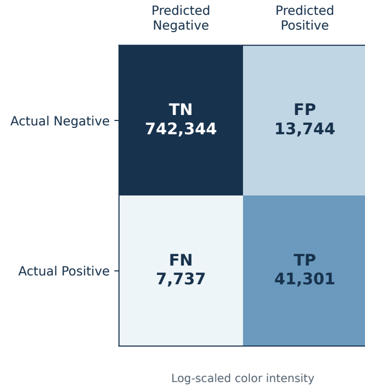
(c) Locked-test confusion matrix
