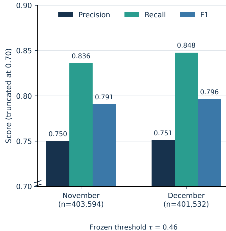
(b) Locked-test monthly stability
