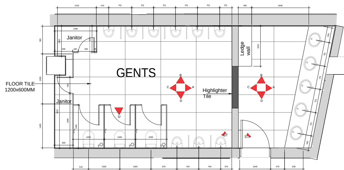
PART PLAN
