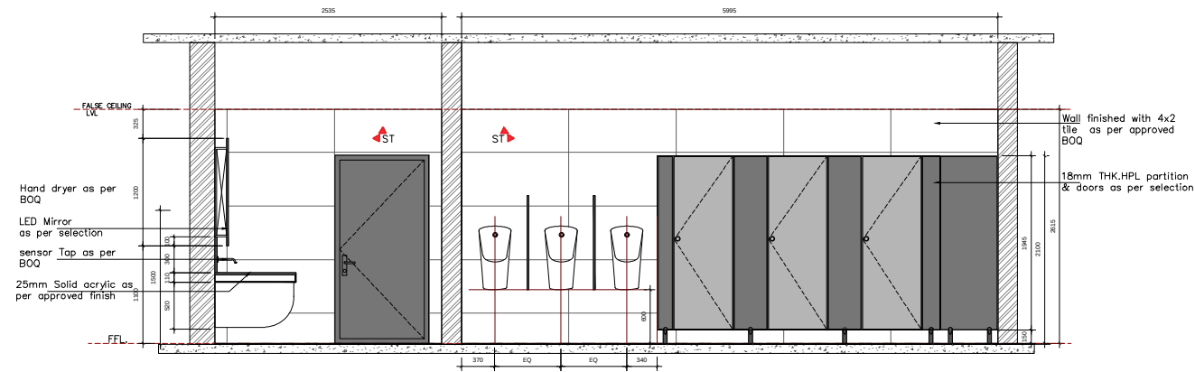
ELEVATION D ALL DIMENSIONS ARE IN MM
