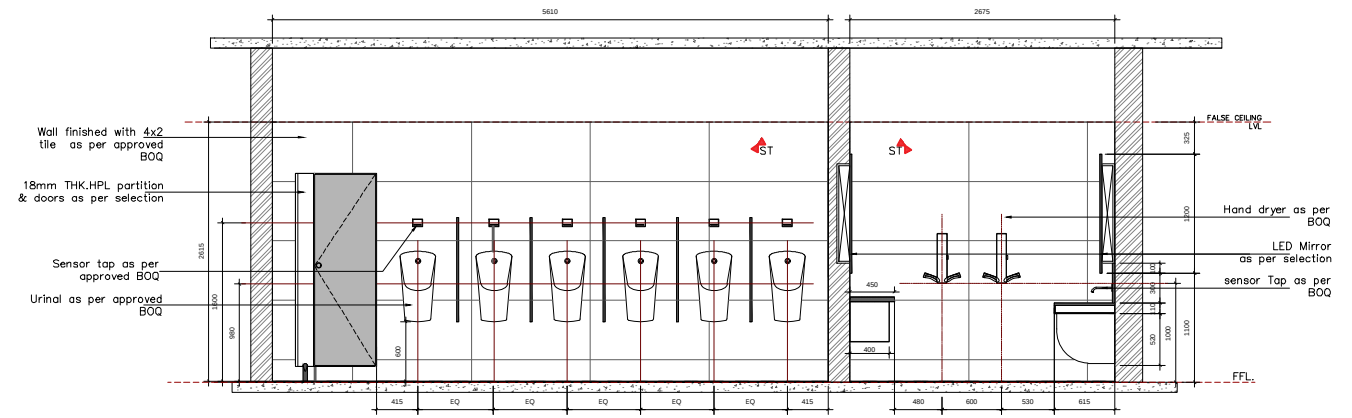
ELEVATION B ALL DIMENSIONS ARE IN MM
