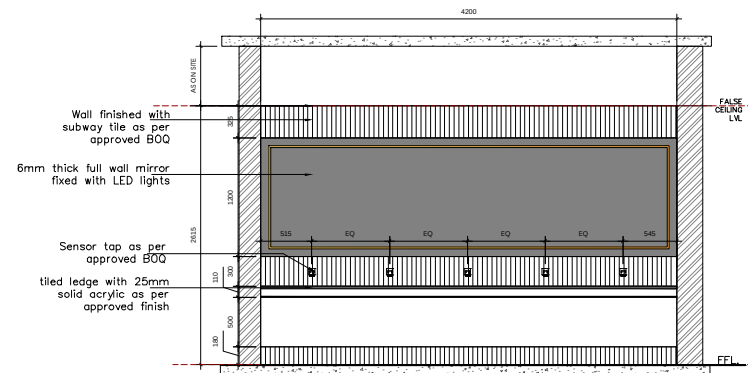
ELEVATION A ALL DIMENSIONS ARE IN MM
