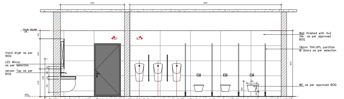
SECTIONAL ELEVATION D' ALL DIMENSIONS ARE IN MM
