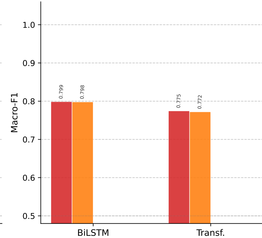
Sequence Models
