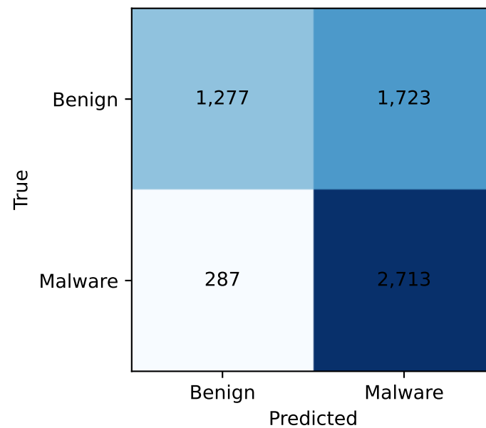
LogisticRegression
