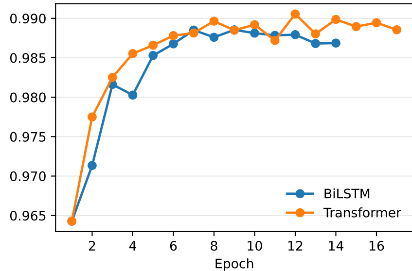
Validation ROC-AUC
