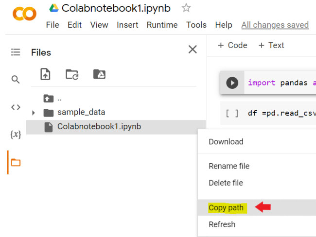
Fig 4. Copy the Path
