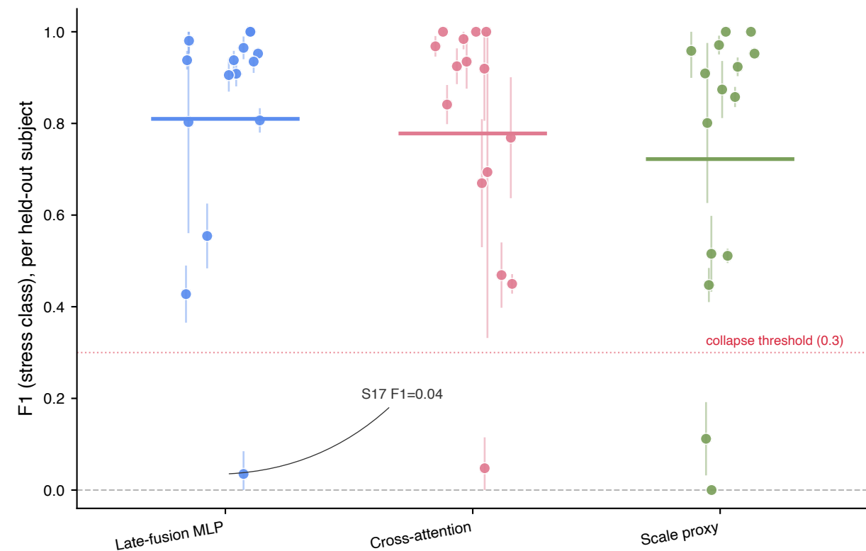
Three failure modes of multi-sensor fusion on WESAD
