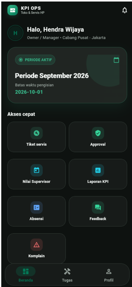
Gambar 31. Beranda Manager
