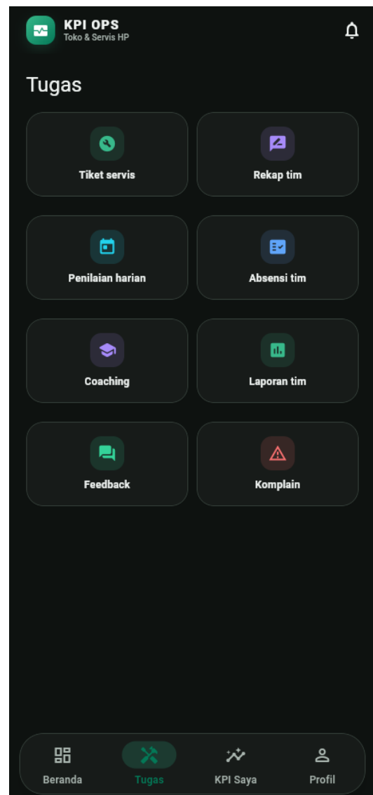
Gambar 6. Tugas Supervisor
