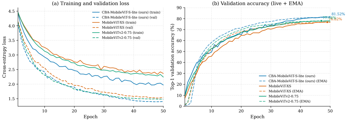
Fig. 8. Training trajectory across 50 epochs. Left: train loss (solid) and validation loss (dashed) for all three lite-budget runs. Right: top-1 validation accuracy (live) and EMA (dashed); best EMA points annotated.
