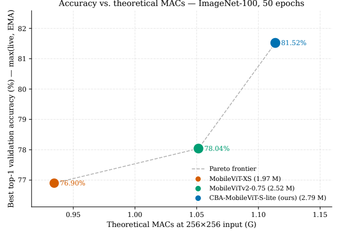
Fig. 7. Accuracy vs. theoretical MACs. ImageNet-100, 50 epochs. y -axis: best top-1 = \max(\text{live}, \text{EMA}) . Point area proportional to parameter count.
