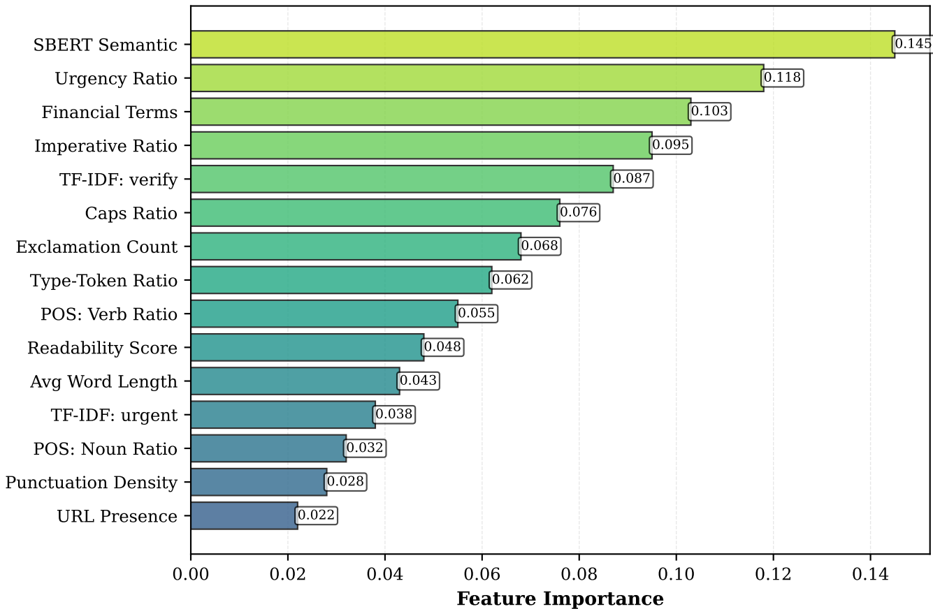
Top 15 Feature Importance (Meta-Learner)
