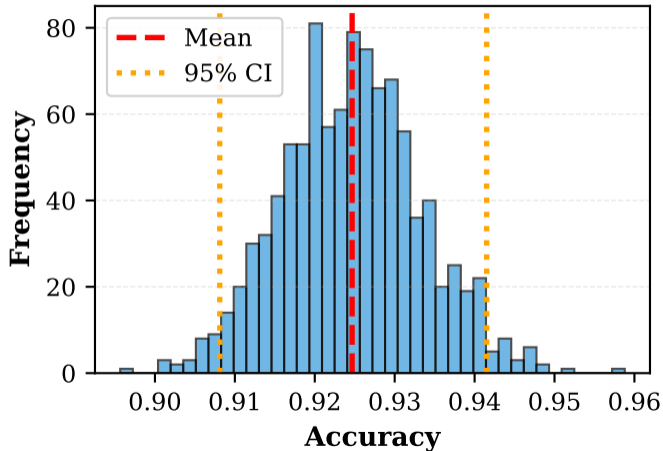
(a) Bootstrap Accuracy Mean: 0.9247 \pm 0.0087
