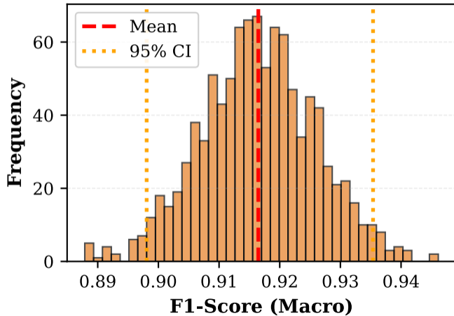
(b) Bootstrap F1-Score Mean: 0.9165 \pm 0.0095
