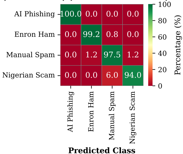
(b) Confusion Matrix (Normalized)
