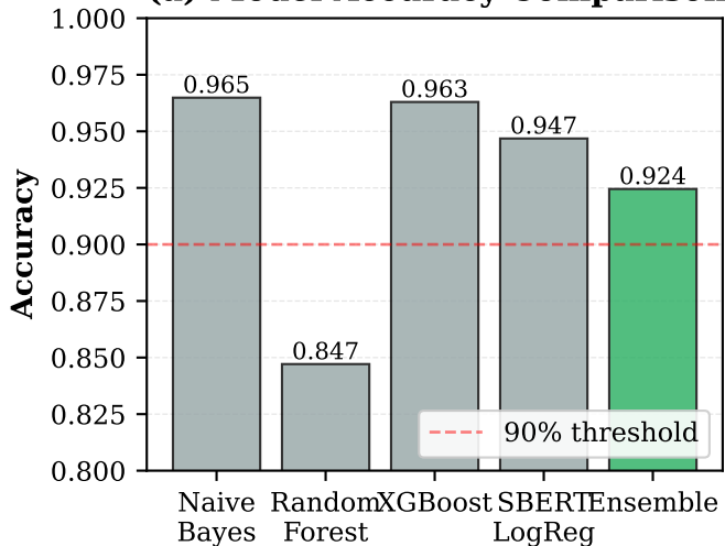
(a) Model Accuracy Comparison
