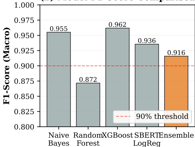
(b) Model F1-Score Comparison
