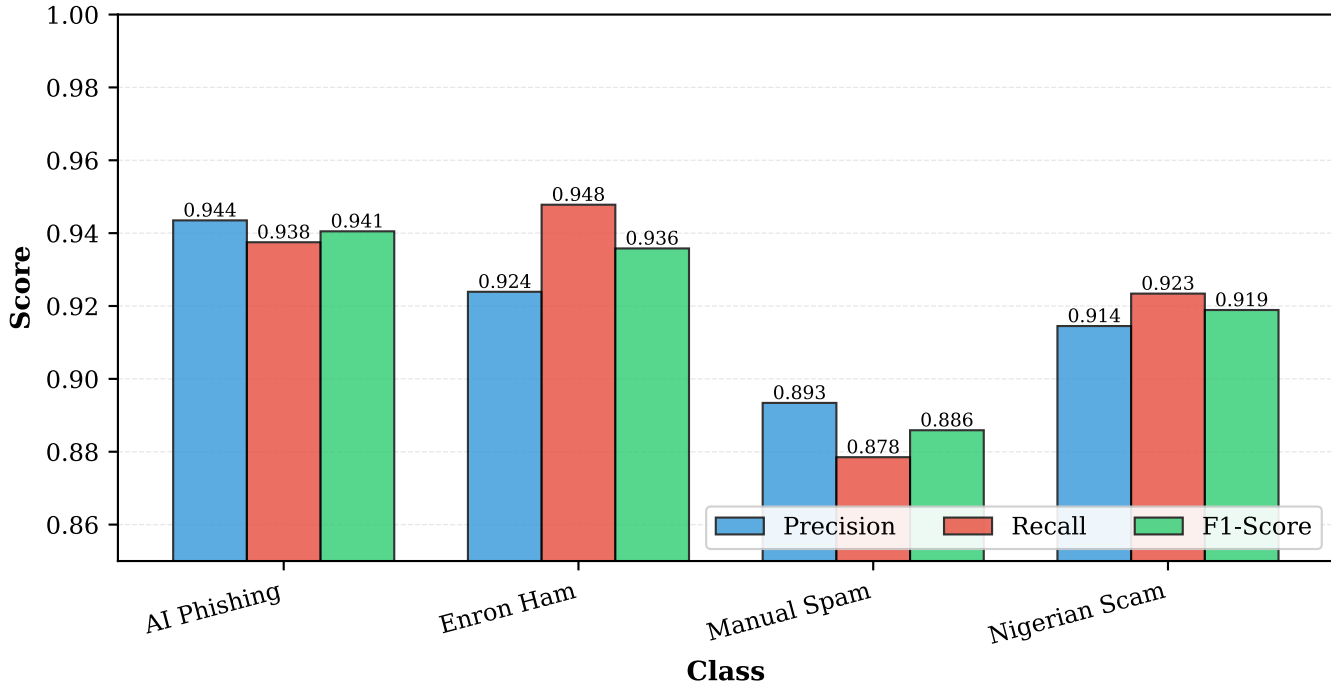
Per-Class Performance Metrics
