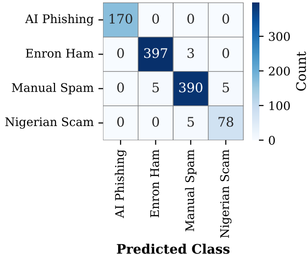
(a) Confusion Matrix (Counts)
