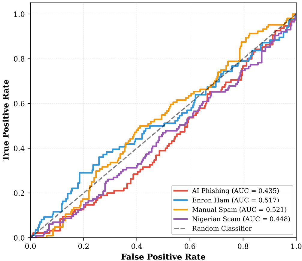
Multi-Class ROC Curves (One-vs-Rest)
