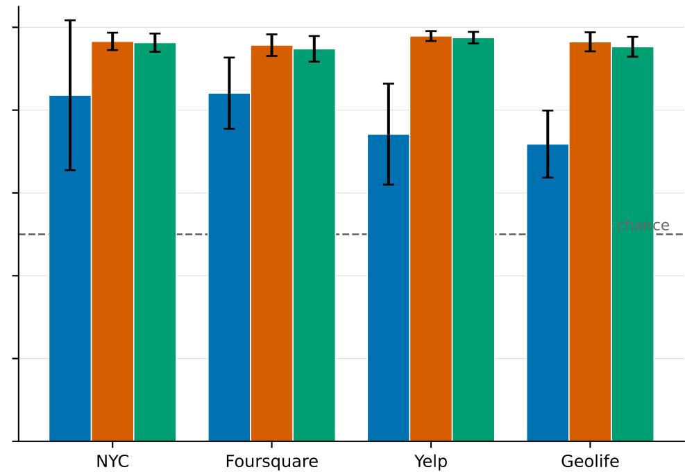
Gradient-poisoning
