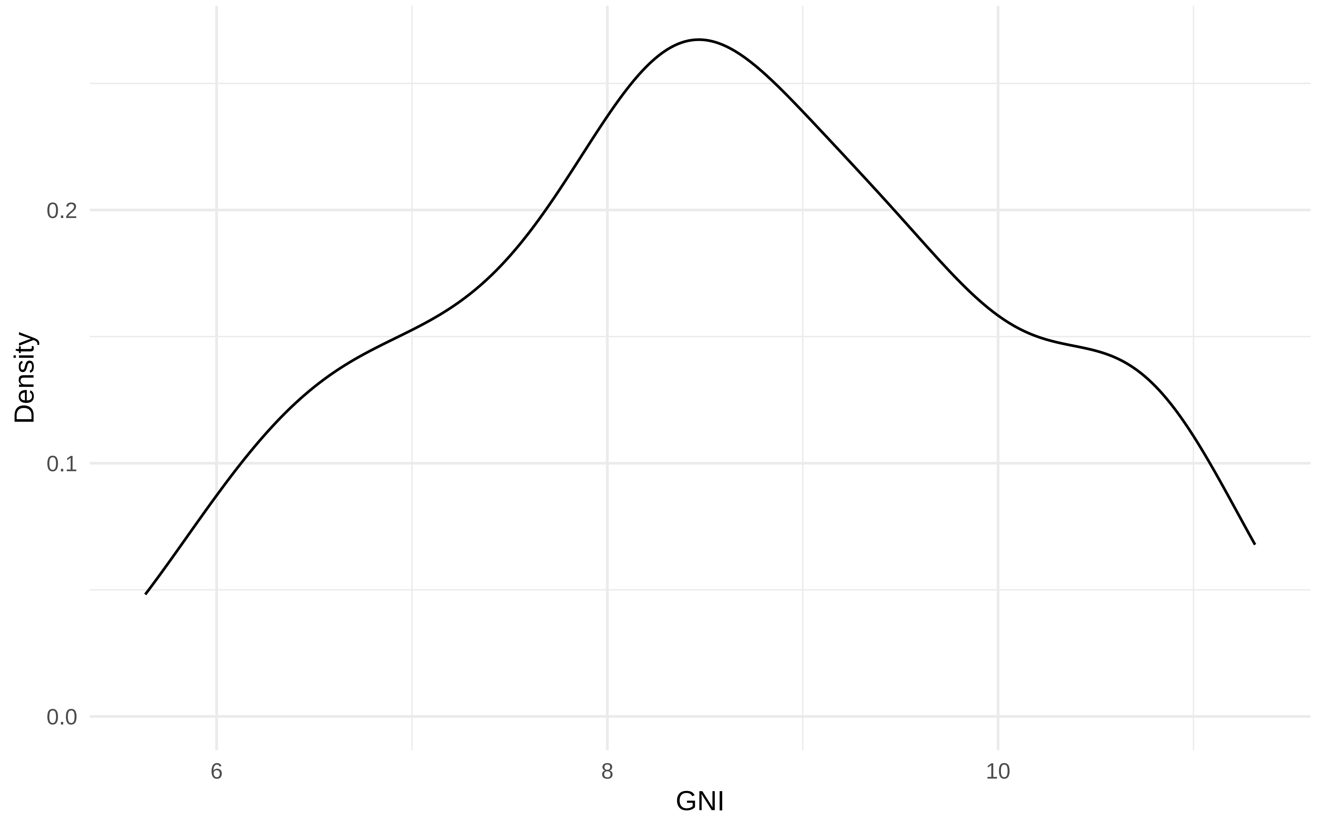
Distribution of log-transformed GNI from 2016 World Bank Data
