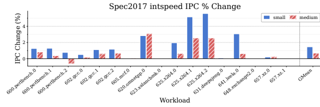
Figure 1: IPC % changes for each CPU model on each intspeed benchmark.
