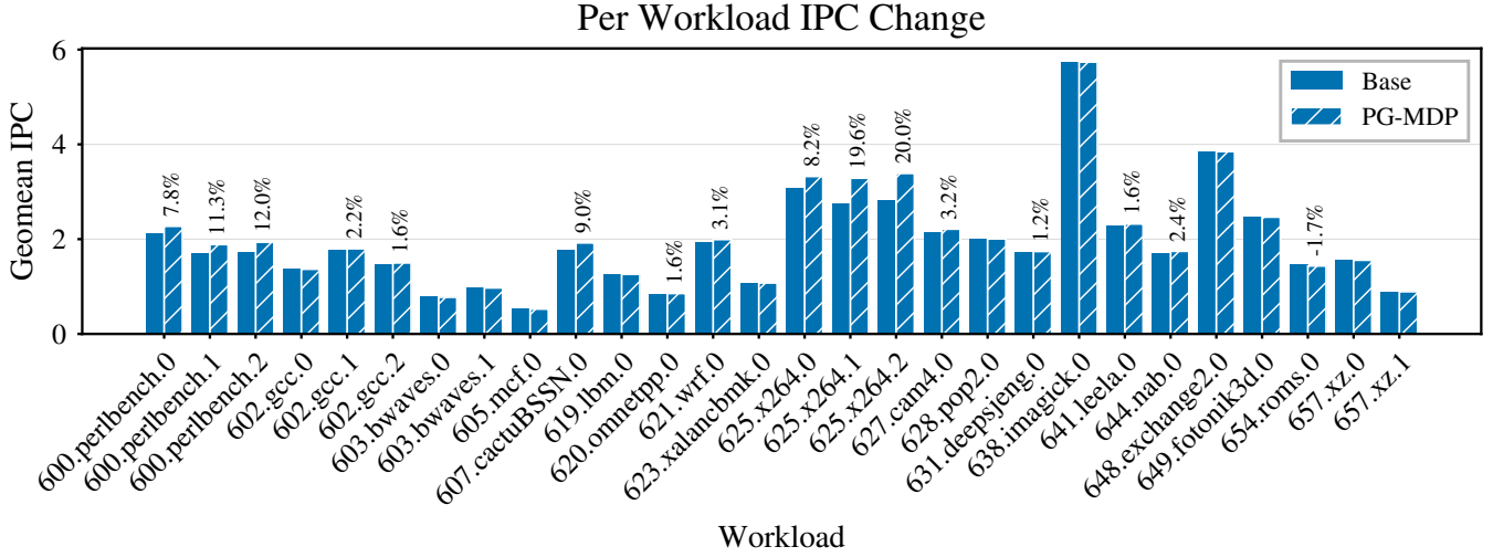
Fig. 4: IPC % improvement with PG-MDP for each workload on the small core configuration. A handful of workloads benefit significantly, whereas others are largely unchanged. Annotations omit percent changes \leq 0.5 .
