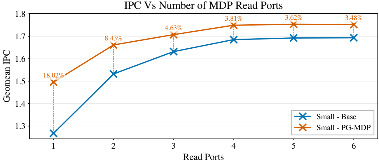
Fig. 7: Geomean IPC of the small core across SPECspeed 2017 against the number of MDP read ports, with and without PG-MDP. Using PG-MDP requires two fewer ports to achieve the same performance as the baseline.
