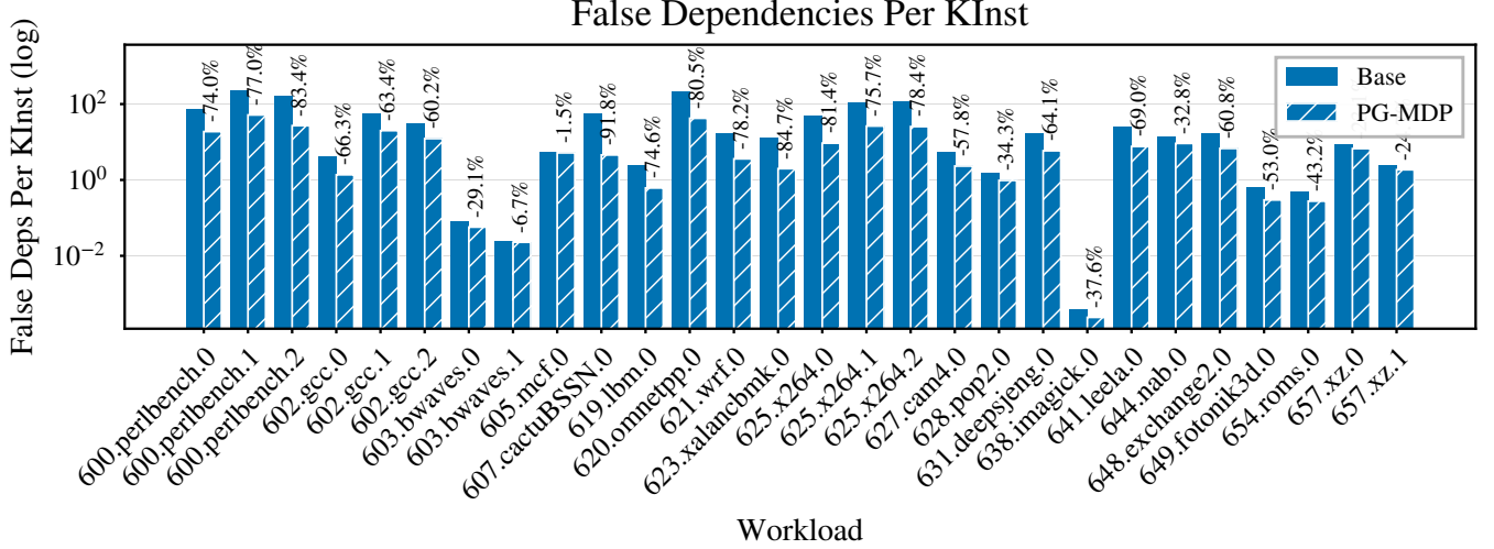
Fig. 6: Percent change of false dependencies per kilo-instruction. PG-MDP benefits workloads most that by default have a higher than average rate of false dependencies, but is still able to cut false dependencies across all workloads.
