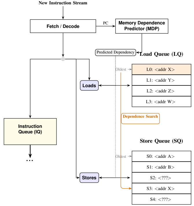
Fig. 2: Diagram of components used to schedule memory operations in out-of-order cores. Memory operations are inserted into the instruction queue according to register dependencies and any predicted memory dependencies, and inserted into the LSQ by program order. When loads execute they search the SQ for forwarding opportunities. When stores execute they search the LQ for memory order violations.
