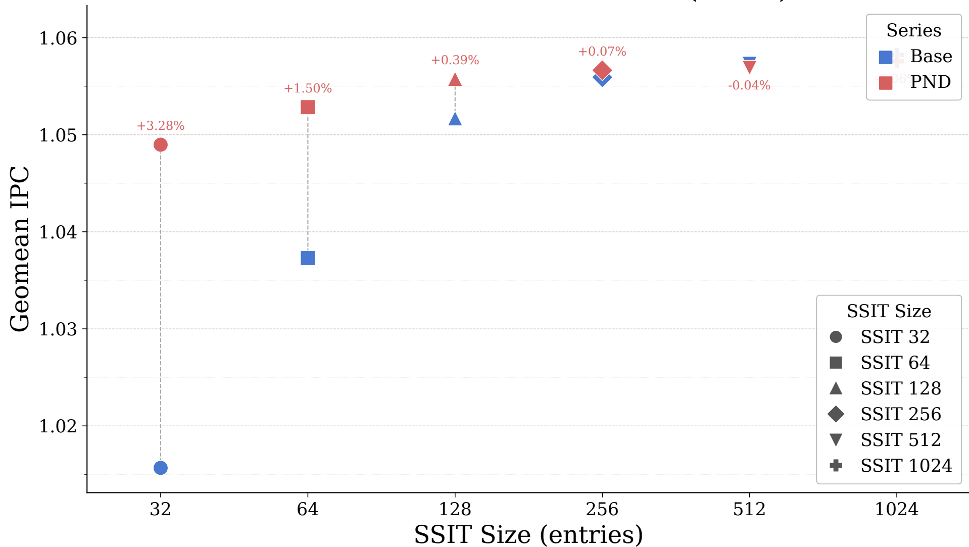
Geomean IPC vs SSIT Size (small)
