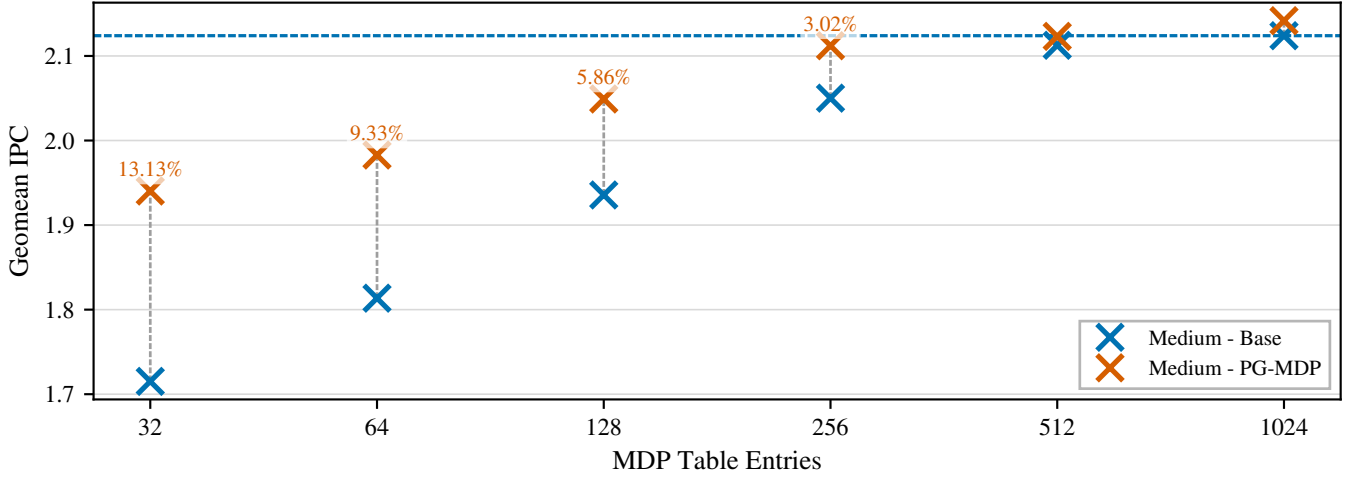
Fig. 5: Base and improved IPC across SPECspeed 2017 for increasing XS Store Set [23] sizes on a medium core (ROB=256). IPC gains increase over the small core, but for the baseline MDP size (256 entries), IPC improvement is still 0.5% smaller.
