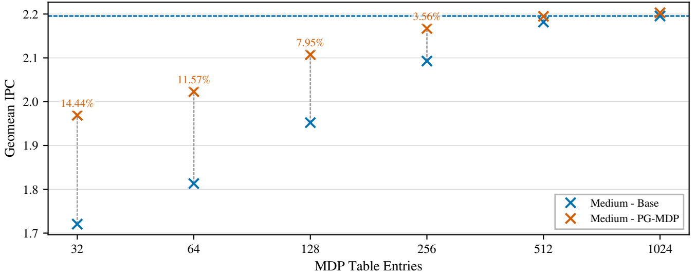
Fig. 6: Base and improved IPC across SPECspeed 2017 for increasing XS Store Sets [28] sizes on a medium core (ROB=256). IPC gains increase over the small core, but for the baseline MDP size (256 entries), IPC improvement is still 1% smaller.
