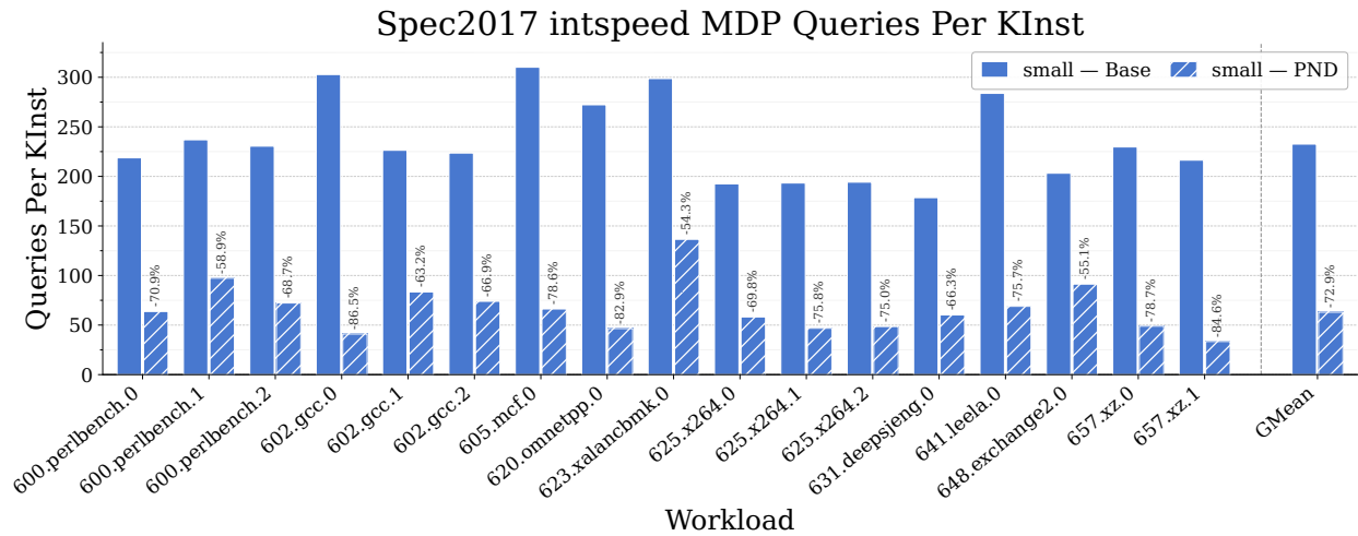
Figure 5: Percent change of MDP queries. Values roughly equal between core sizes.
