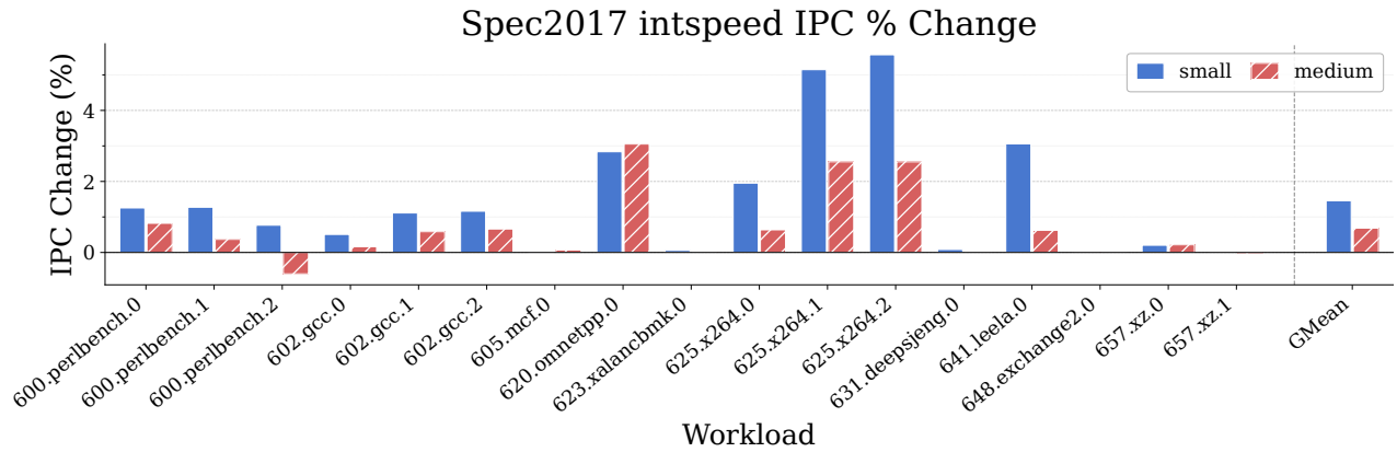
Figure 2: IPC % changes for each CPU model on each intspeed benchmark.
