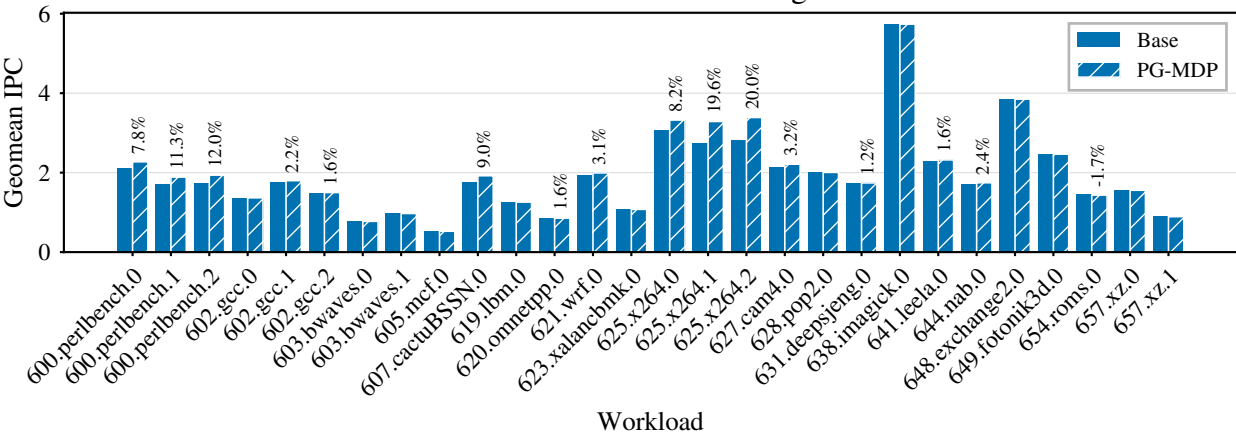
Per Workload IPC Change
