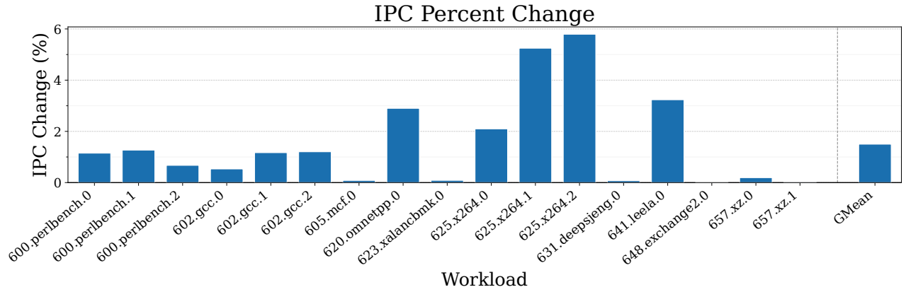
Figure 5: TODO: overview the important trend in each figure caption. IPC % changes for each CPU model on each intspeed workload.
