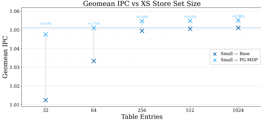
Figure 8: SPEC2017 CPU intspeed geomean IPC with and without PG-MDP for varying XS Store Set sizes. PG-MDP is able to effectively improve small predictor performance to within levels near-equal to large predictors for both a small and medium sized core.
