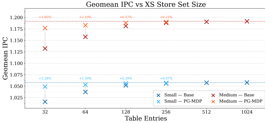
Figure 3: SPEC2017 CPU intspeed geomean IPC with and without PG-MDP for varying XS Store Set sizes. PG-MDP is able to effectively improve small predictor performance to within levels near-equal to large predictors for both a small and medium sized core.
