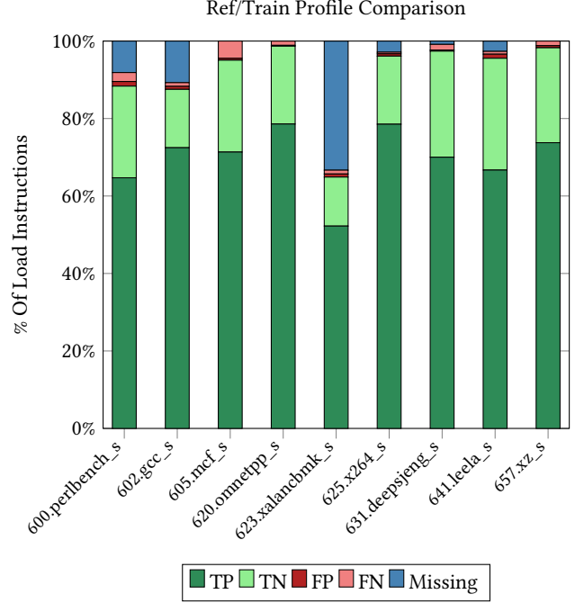
Figure 3: Comparison of labelled (static) loads between profiles generated from intspeed train and ref inputs with a store distance threshold of 8. Most labels are true positives/negatives when compared to the reference inputs, and very few are false positives.
