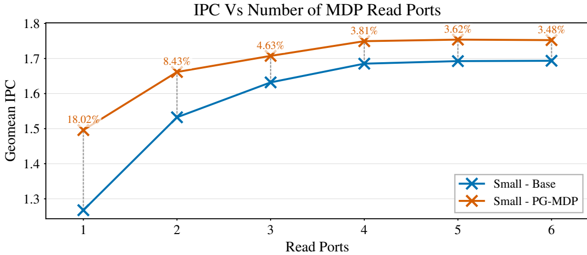
Figure 7: Geomean IPC of the small core across SPECspeed 2017 against the number of MDP read ports, with and without PG-MDP. Using PG-MDP requires two fewer ports to achieve the same performance as the baseline.
