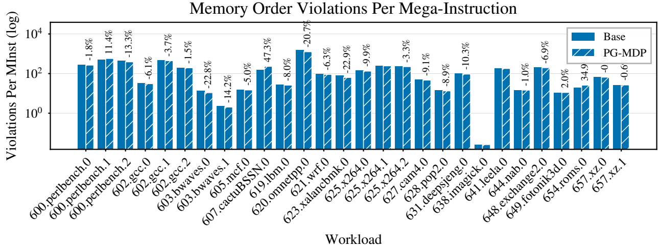
Figure 6: Percent change of memory order violations per Mega-instruction. Although relative % changes are high, absolute values remain low.
